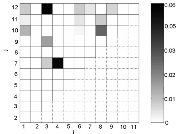
Fig. 13 – Second-order indices S_{ij} for the IPT with the tolerance level of \varepsilon = 0.07 .
