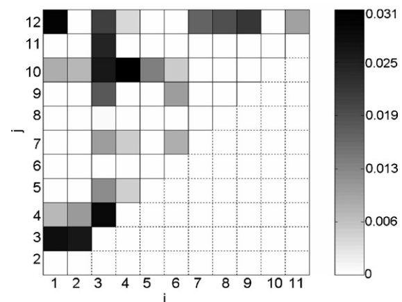
Fig. 15 – Second-order indices S_{ij} for the IPT with the tolerance level of \varepsilon = 0.2 .
