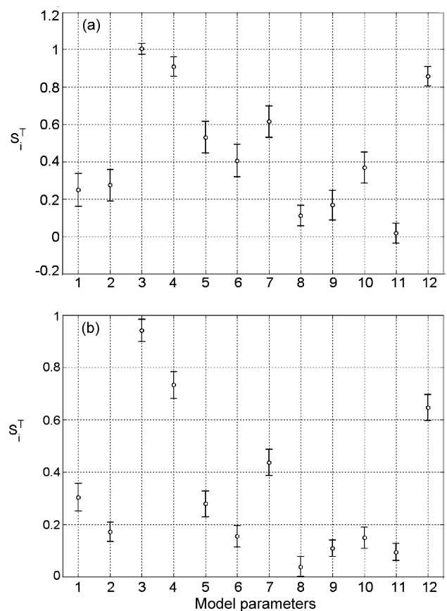
Fig. 14 – The total sensitivity indices for the IPT on the tolerance level: (a) \bar{\varepsilon} = 0.2 and (b) \bar{\varepsilon} = 0.5 . Bars show 95% confidence intervals computed by the bootstrap technique.
