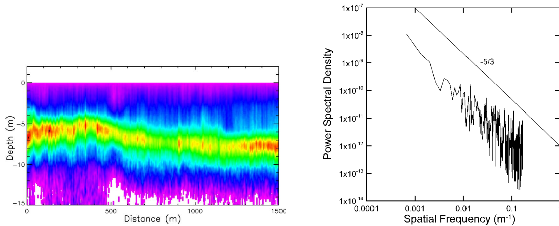
Fig. 3. Echogram of a segment of phytoplankton layer (left) and the power spectral density of the backscattering magnitude at the peak (right). Right panel also shows the -5/3 power law characteristic of a turbulent spectrum.
