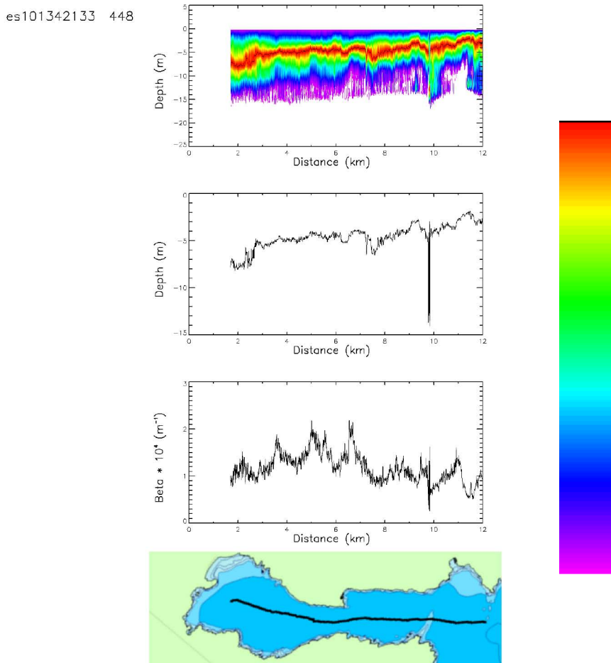
Fig. 2. Stacked plot of a typical lidar transect, plotted as functions of distance from the head of the sound. Top panel is the normalized lidar echogram for the co-polarized channel, plotted using the color bar to the right. Next panel is the depth of the peak return in each lidar pulse. Third panel is the cross-polarized volume scattering coefficient (at a scattering angle of \pi radians) for the peak returns. Bottom panel is a chart of the sound, rotated to align with the other panels, showing the transect flight track.
