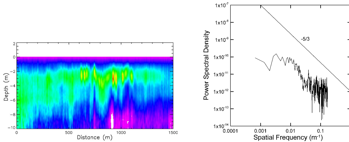
Fig. 4. Echogram of a segment of zooplankton layer (left) and the power spectral density of the backscattering magnitude at the peak (right). Right panel also shows the -5/3 power law characteristic of a turbulent spectrum.
