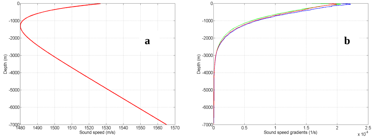
Figure 1. Average sound speed profile (a) and RMS horizontal sound gradients (b). Depth dependences of \langle (\partial c / \partial x)^2 \rangle^{1/2} (blue) and \langle (\partial c / \partial y)^2 \rangle^{1/2} (red) calculated from Monte Carlo simulations of internal wave fields agree well with the theoretical profile (green). [Sound speed has a single minimum of 1480 m/s at depth z = -1300 m and equals 1528 m/s and 1565 m/s at z = 0 and z = -7000 m. RMS range- and cross-range components of the sound speed gradient have maxima of about 2 \text{ s}^{-1} at z \approx -40 m and decrease to zero with increasing depth.]
