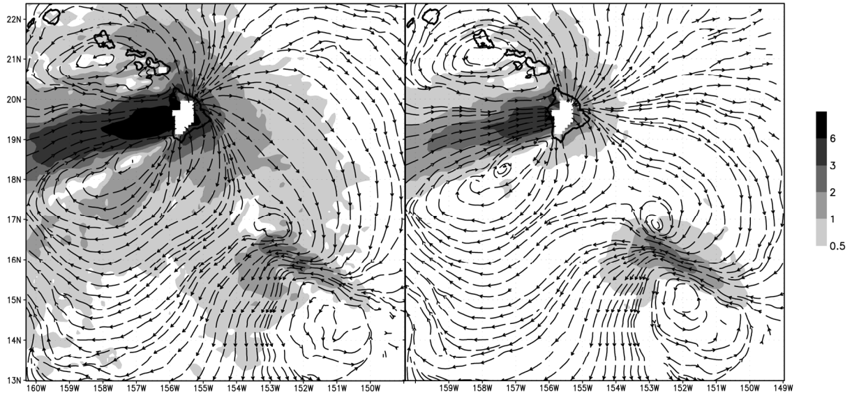
Fig. 11 Tropical storm 850 hPa to 700 hPa (left) and hurricane 850 hPa to 400 hPa (right) steering flow difference (Big Island – no Big Island) in \text{m s}^{-1} averaged from hours 12 to 24 for a simulation of Hurricane Flossie (2007).
