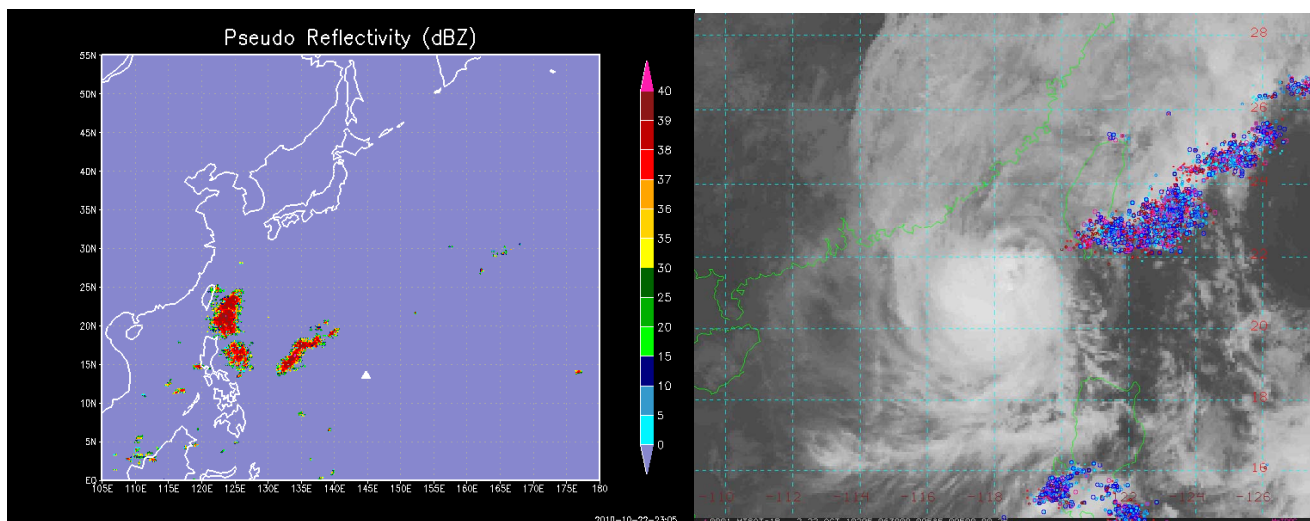
Fig. 3. (Left) Example of a pseudo reflectivity product on 22 October 2010 at 2300 UTC showing estimates of radar reflectivity associated with a rainband from typhoon Megi. (Right) Lightning in vigorous rainband approaching Taiwan. Positive flashes are shown in red shades and negative flashes in blue shades for 0600 UTC, 22 October 2010.
