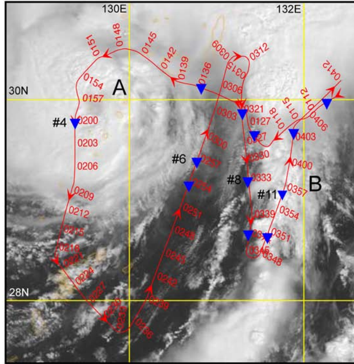
(a) 2008-09-18 01:41UTC MODIS VIS and NRL P-3 Flight track
