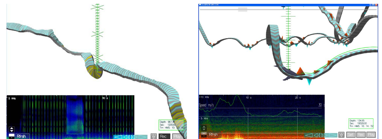
Figure 1. Left: the acoustic spectrogram from a beaked whale foraging at 967m depth revealing clicks and buzzes. Data courtesy of Brandon Southall. Right: the typical acoustic signature of a lunging humpback feeding on krill. The overlaid plot shows speed estimated from flow noise.
