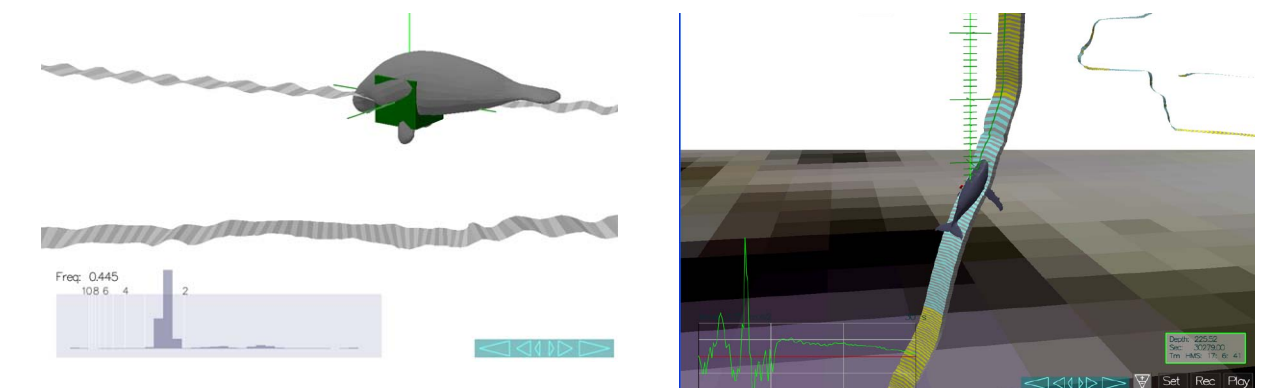
Figure 2. Left: a TrackPlot image of a Florida manatee. The insert shows one of the plot options based on a fourier analysis of the residual accelerometer data. Right: the inset plot shows the residual acceleration attributable to a vertical lunge by a humpback.
