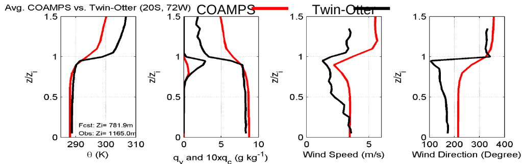
Figure 4. Evaluation of COAMPS real-time forecast using Twin-Otter soundings from VOCALS.
