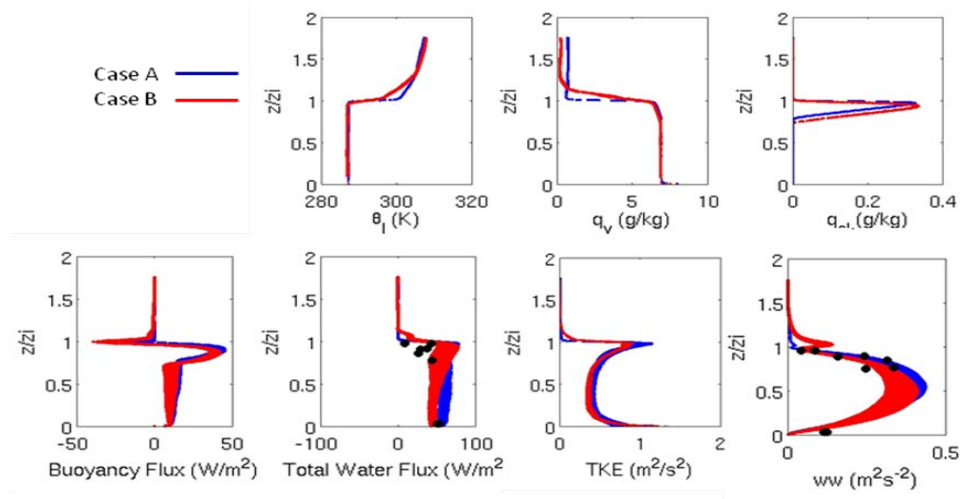
Figure 5. LES profile of mean state; (top), buoyancy flux, the total water flux, the turbulence kinetic energy (TKE) and the vertical velocity variance from the LES cases during the 4 th hour bottom). The total water flux and the vertical velocity variance calculated from aircraft observations are marked as black dots.
