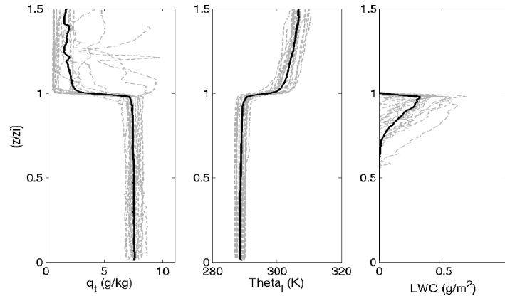
Figure 1. Profiles scaled by the PBL heights of a) total-water specific humidity ( \text{g/kg} ); b) liquid water potential temperature ( \text{K} ); and c) LWC ( \text{g m}^{-2} ) The gray lines are for individual flights, and the black solid lines show the averaged soundings.
