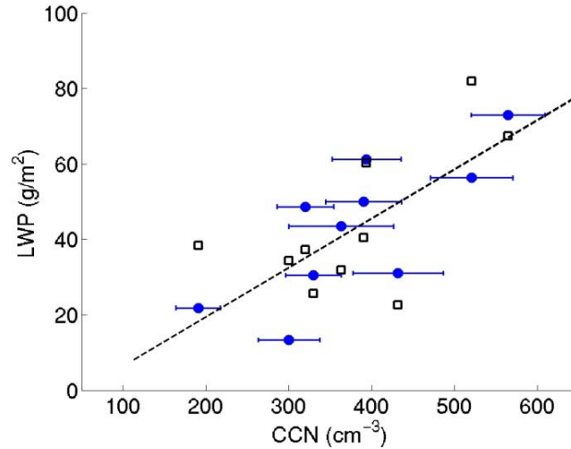
Figure 2. LWP as a function of sub-cloud CCN concentrations for selected 10 flights. Blue solid symbols are from aircraft profiles. The error bars through these symbols indicate the standard deviation of CCN. Open symbols are averages from GOES retrievals within radii of 20 km. Line is the best fit to the aircraft LWP estimates.
