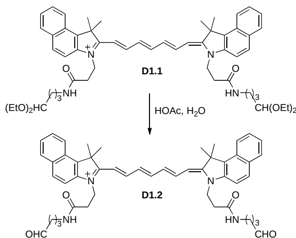
Scheme D1. Synthesis of a Cypate-bis(aldehyde).
