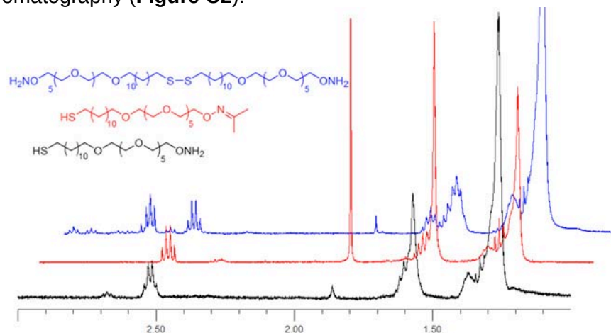
Figure C2. Comparison of the ^1\text{H} NMR spectra for the representative thiol-aminoxy diblock spacer 12/6 (black), its corresponding acetone adduct (red), and its disulfide dimer (blue).
