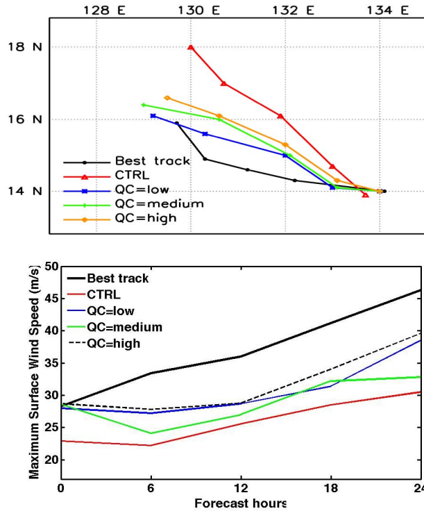
Figure 2. Time evolution of the storm track (top panel) and maximum surface wind ( \text{m s}^{-1} ) (bottom panel) of Typhoon Jangmi from control experiment (CTRL, without assimilation of radar data), experiments with assimilation of both the reflectivity and radial velocity under various quality levels of the data, compared with the JTWC best track data during 0000 UTC 25 to 0000 UTC 26 September 2008.
