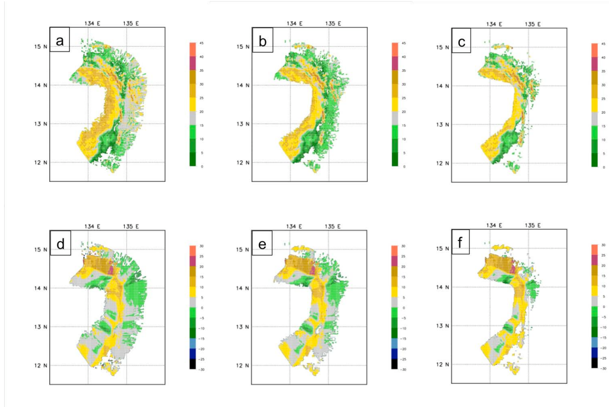
Figure 1. Radar reflectivity (dbz, a-c) and radial velocity ( \text{m s}^{-1} , d-f) at 0.5 km height level with different quality control (QC) levels around 0000 UTC 25 September 2008. (a) and (d): Low QC level; (b) and (e): Medium QC level; (c) and (f): High QC level.
