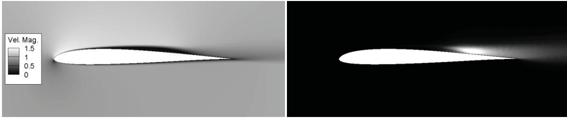
Figure 4. 2D Time and spanwise averaged velocity magnitude (right) and turbulent kinetic energy (left).
