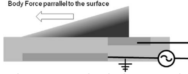
Figure 1. Diagram of a DBD plasma actuator. Two electrodes (the upper powered and the lower grounded) are asymmetrically separated by a dielectric material. During operation, the gas region from the powered to grounded electrodes is weakly ionized.
