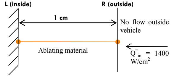
Figure 1. Schematic of 1-D thermal ablation problem (material is carbon phenolic)
