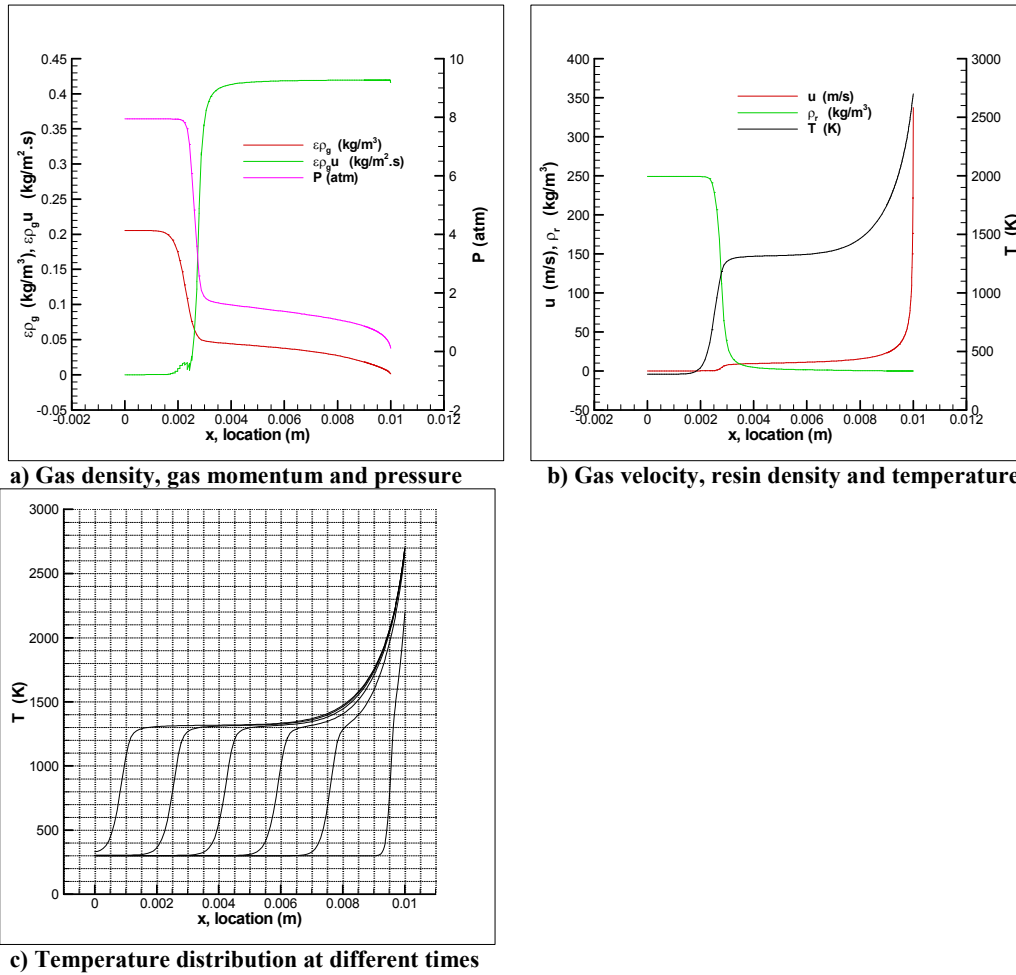
Figure 6. Top two plots a) and b) show all solution variables for Arc-jet case with D = 0 at time = 4 sec. a) shows gas density, \epsilon \rho_g , gas momentum, \epsilon \rho_g u and pressure, P ; b) shows gas velocity, u , resin density, \rho_r , and temperature, T ; and c) shows temperature distribution within the domain at times = 0.1, 1, 2, 3, 4, and 5 sec.
