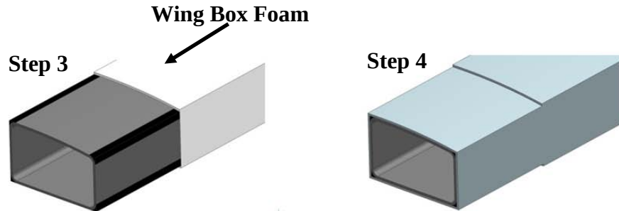
Figure 31. Attach the Joiner Block Layup to the Wing Box Foam and Wrap Assembly in E-Glass Cloth [23]
