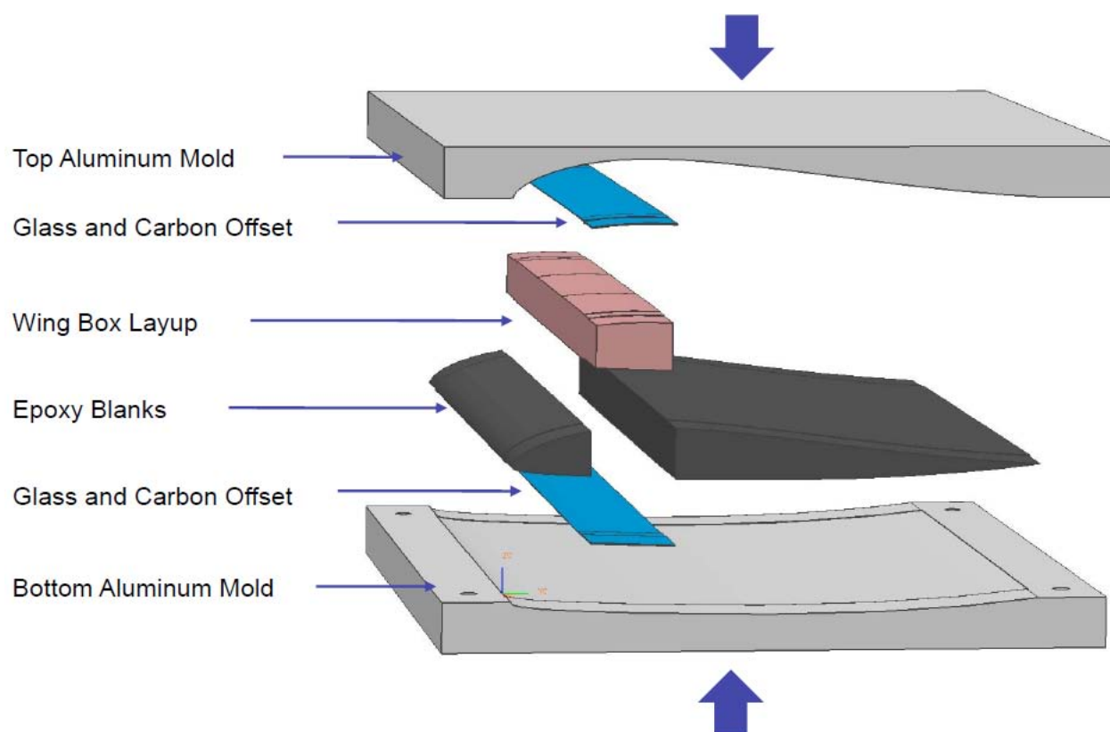
Figure 34. Wing Aluminum Mold [5]
