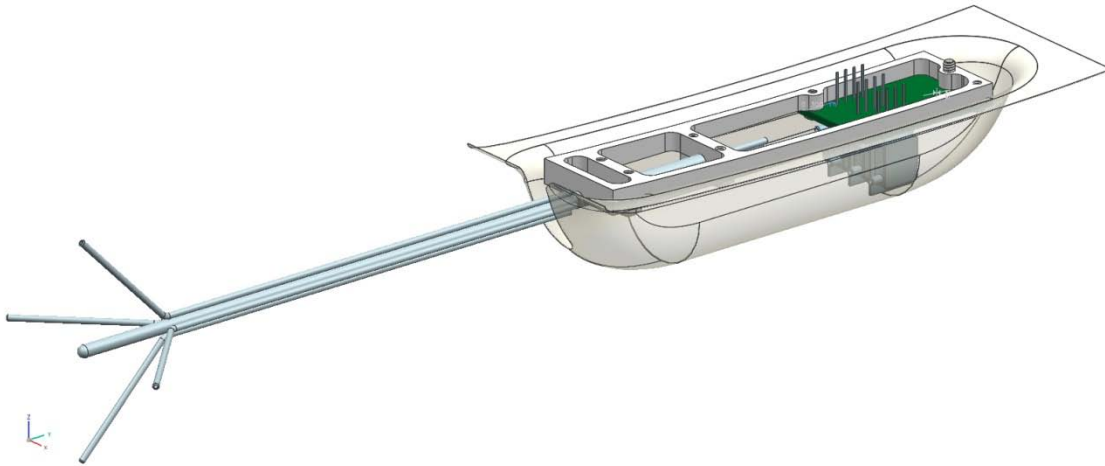
Figure 63. 5 Hole Pitot Probe
