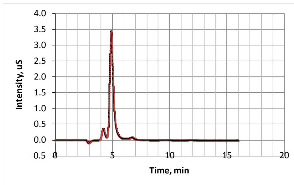
Figure 9. IC chromatogram of catholyte (Anode: Ir, 3\text{mg}/\text{cm}^2 , cathode: Pt, 1.5\text{mg}/\text{cm}^2 , anolyte: seawater, catholyte: fresh water).
