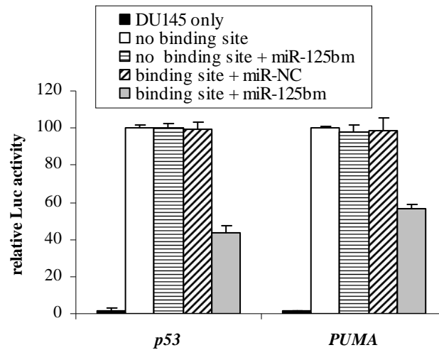
Fig. 1. Luciferase analysis of miR-125b binding to the 3'UTRs of p53 and PUMA in DU145 cells. Individual truncated 3'UTRs of p53 and PUMA were used as controls (no binding site) in these experiments. The assay was repeated three times with each assay being performed in three wells and similar results were obtained each time. The representative results are shown as M \pm SD ( n = 3 ).
