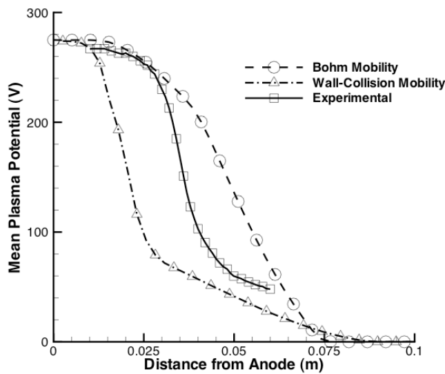
Figure 16. Centerline profiles of plasma potential for the P5 Hall thruster (from Koo and Boyd [56]).
