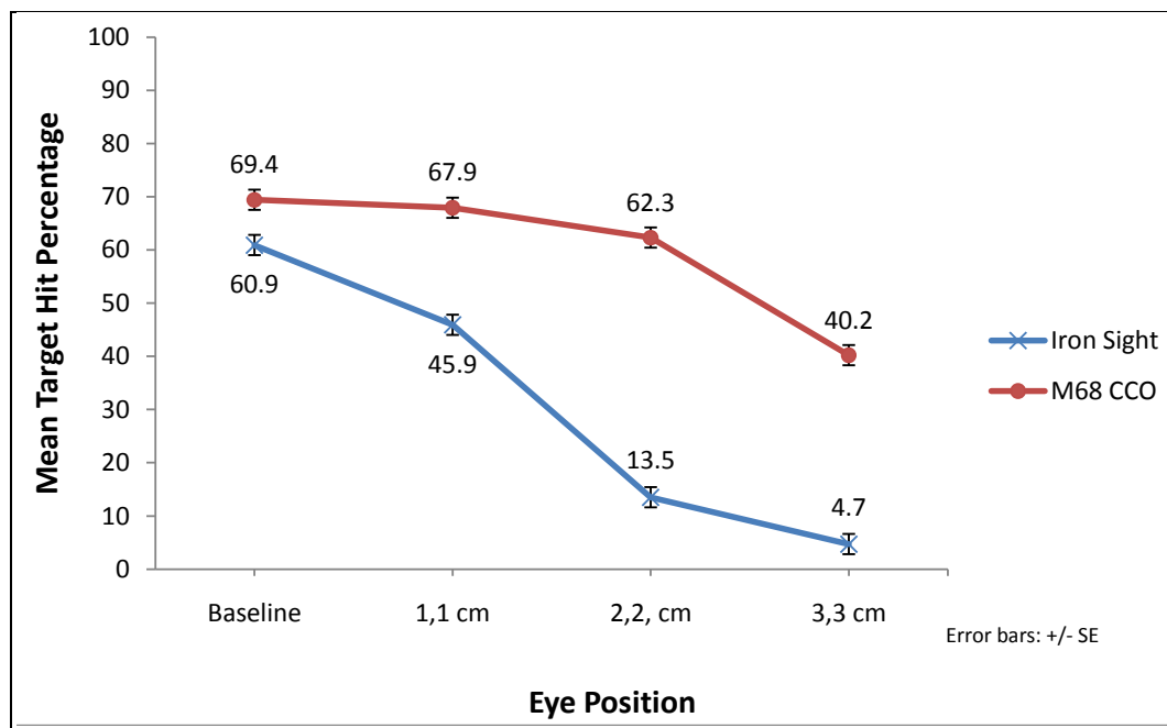
Figure 8. The effect of eye position condition \times sight on mean target hit percentage for the aimed fire shooting task.
