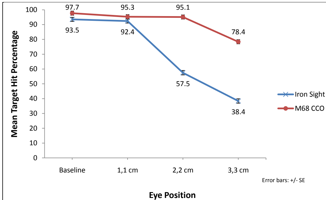
Figure 11. The significant interaction effect of eye position x sight on mean target hit percentage for the reflexive firing shooting task.
