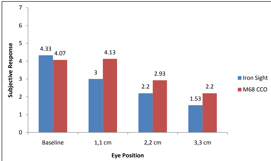
Figure 15. Rating of cheek pressure required.
