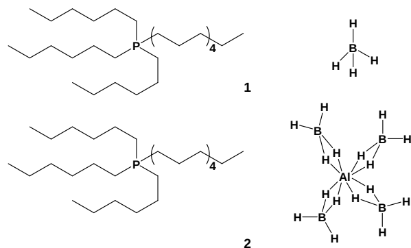
Scheme 2. Novel borohydride ILs ( 1 ) (top), ( 2 ) (bottom).
