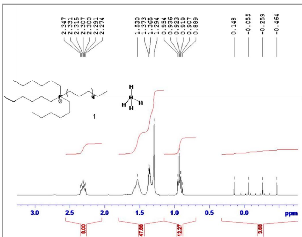
Figure S2. ^1H NMR of (1) in CD_2Cl_2 (expanded).
