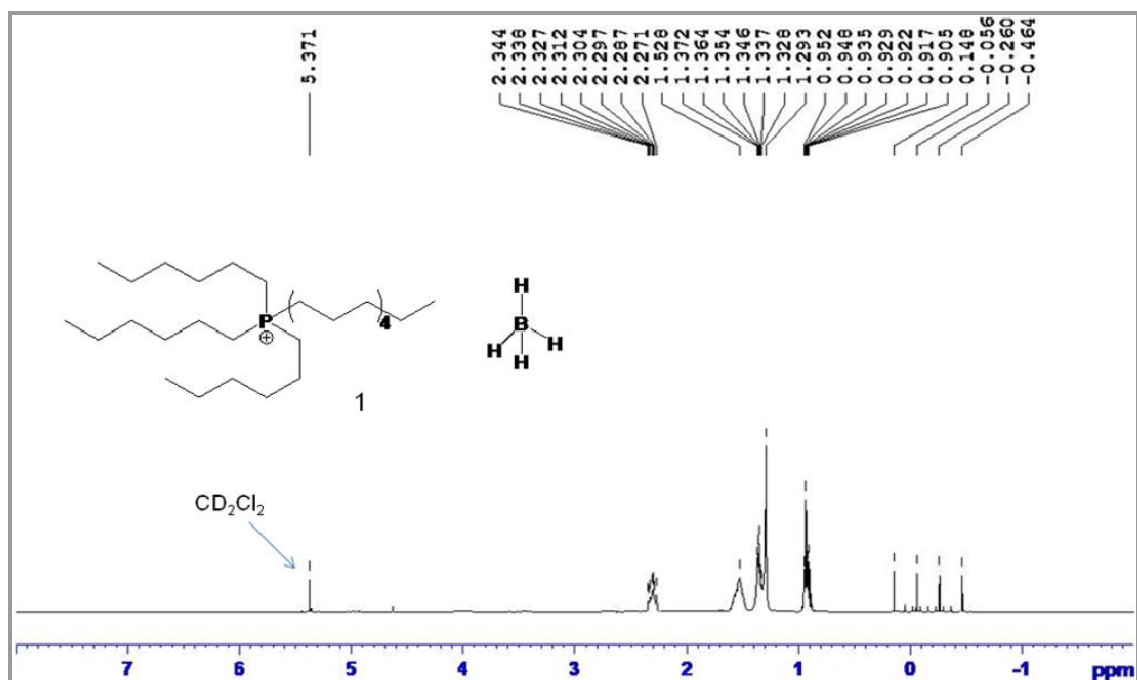
Figure S1. ^1H NMR of (1) in CD_2Cl_2 .
