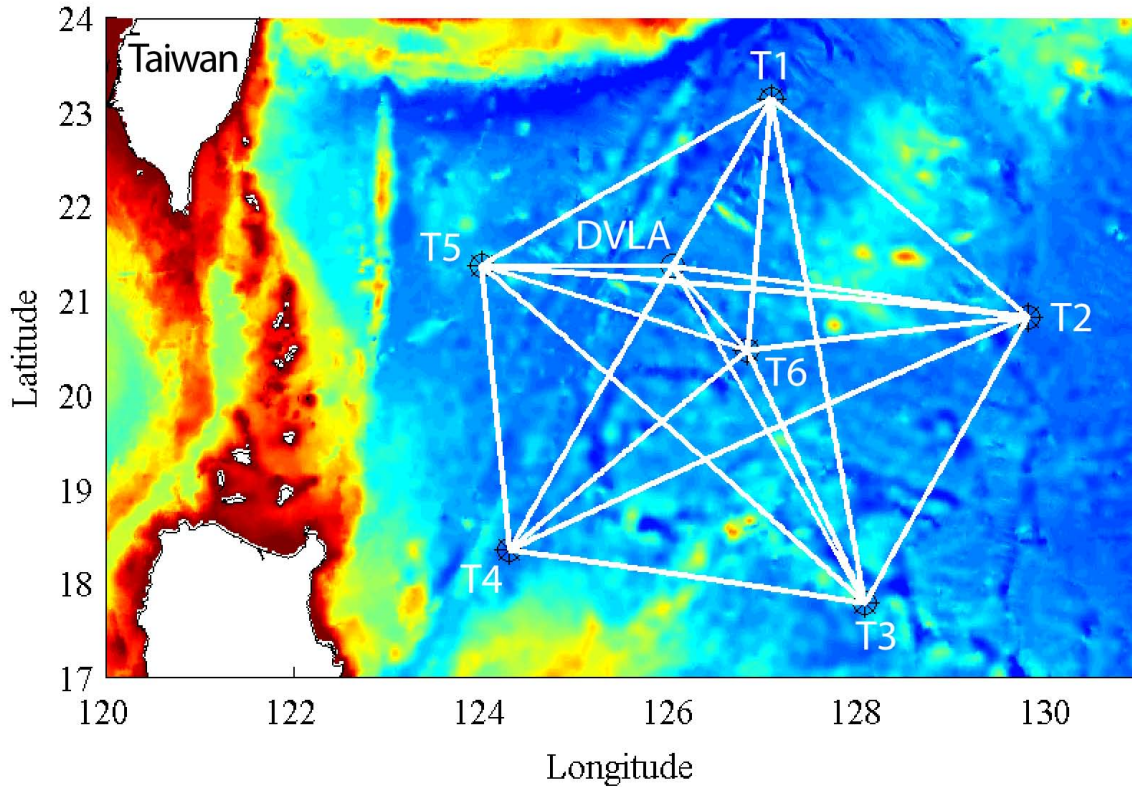
Figure 1. Overall mooring geometry of the 2010–2011 Philippine Sea Experiment, consisting of five 250-Hz acoustic transceivers arranged in a pentagon with a sixth transceiver in the center (T1, T2, ... T6) and a new DVLA receiver. The array radius is approximately 330 km.
