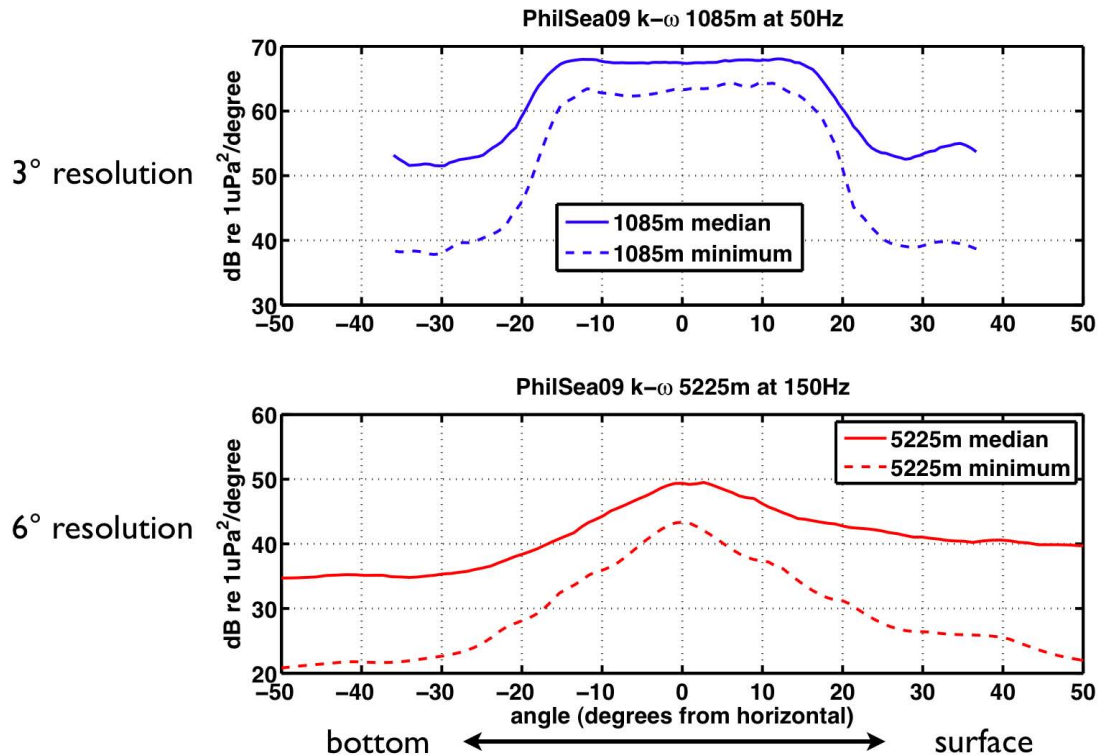
Figure 4. Vertical ambient noise distributions at 1085 m depth (near the sound channel axis) at 50 Hz and at 5225 m depth (below the surface conjugate depth) at 150 Hz. The median and minimum noise levels over the approximately one-month duration of PhilSea09 are shown.
