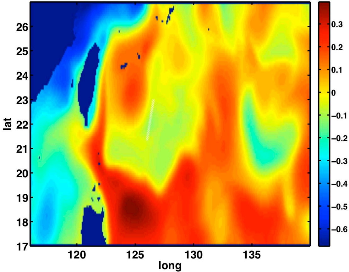
Figure 2. Sea surface height anomaly (m) on 23 April 2009 from a regional implementation of the MITgcm ocean circulation model in the northern Philippine Sea. The sharp zonal gradient in sea-surface height immediately east of Taiwan is associated with the northward-flowing Kuroshio Current. The features in the interior of the northern Philippine Sea are associated with the energetic mesoscale eddy field in the area. The white line at about 22°N, 125°E is the acoustic propagation path from the moored source to the DVLA during PhilSea09.
