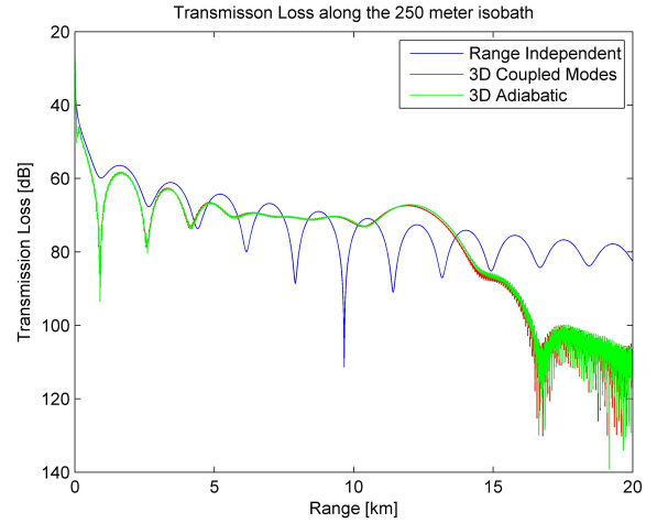
Figure 4: Transmission Loss [dB] for the coupled-mode and adiabatic solutions shown in the first two panels of figure 3 as a function of y for x=1.8 km with the range independent solution for comparison.
