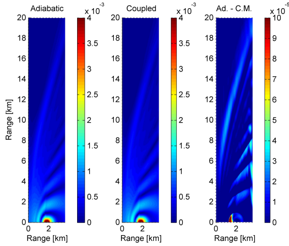
Figure 3: Pressure [Pa] at a depth of 20 meters. The left panel shows the adiabatic solution, the center panel shows the coupled-mode solution, and the right panel is the difference between the adiabatic and coupled-mode solutions.
