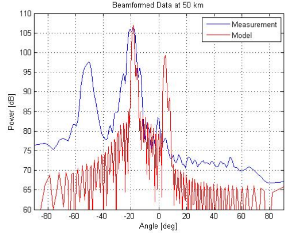
Figure 6: Beam power from measured (blue) and modeled (red) data for a source 50 km north of the array location.
