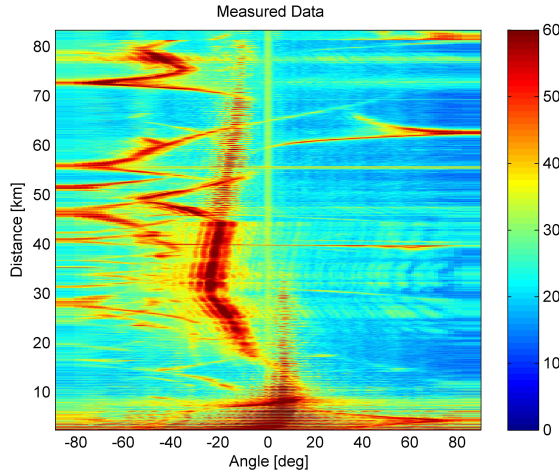
Figure 5: Narrowband BTR of the measured data. The time axis of the BTR has been replaced by distance north of the array location.
