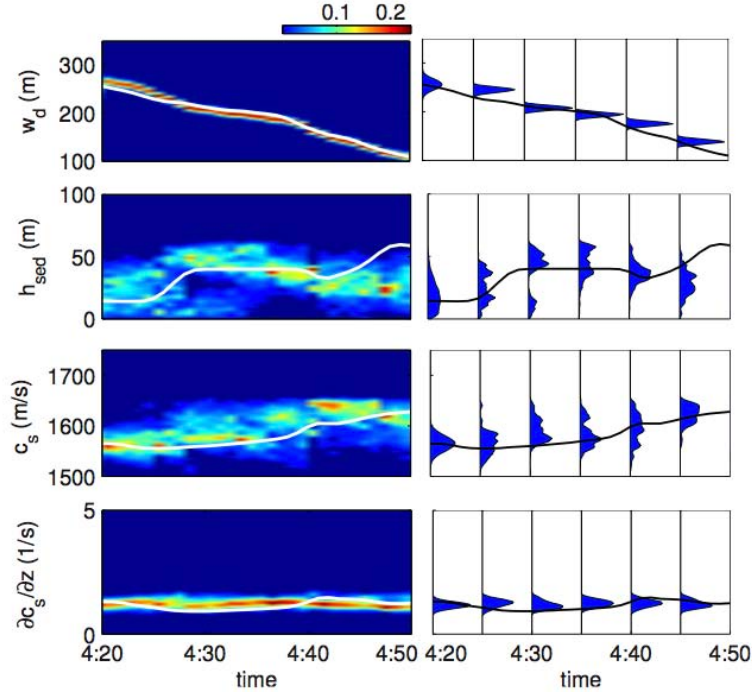
Figure 5. Evolving marginal posterior PDFs for the geoacoustic parameters: (a) water depth ( w_d ), (b) sediment thickness ( h_{sed} ), (c) sediment sound speed at the water-sediment interface ( c_s ), and (d) sediment sound speed gradient ( \partial c_s / \partial z ). Vertical slices of the PDFs are given at 5 min intervals. Solid lines represent the true values.
