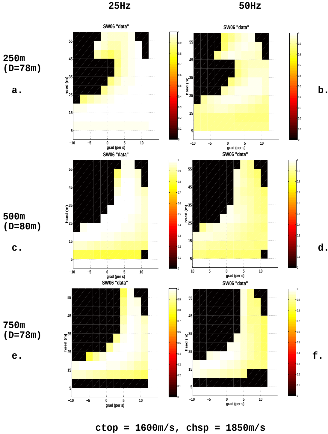
Figure 3: Plots of the MFP values higher than 0.8 (light shades) for multiple frequencies as shown and multiple ranges as shown. The fixed parameters have been set to the “true” values: c_{top} = 1600\text{m/s} , c_{hsp} = 1850\text{m/s} , with D as indicated per subplot.
