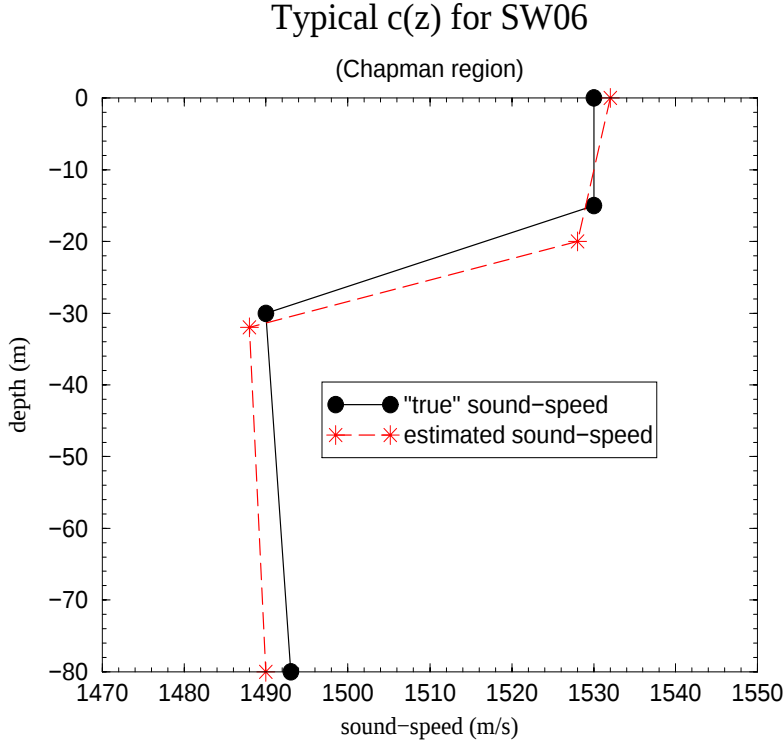
Figure 2: The ocean sound-speed profiles for the simulated SW06 scenario. “True” is the solid curve, the dashed curve is used in the inversions.
