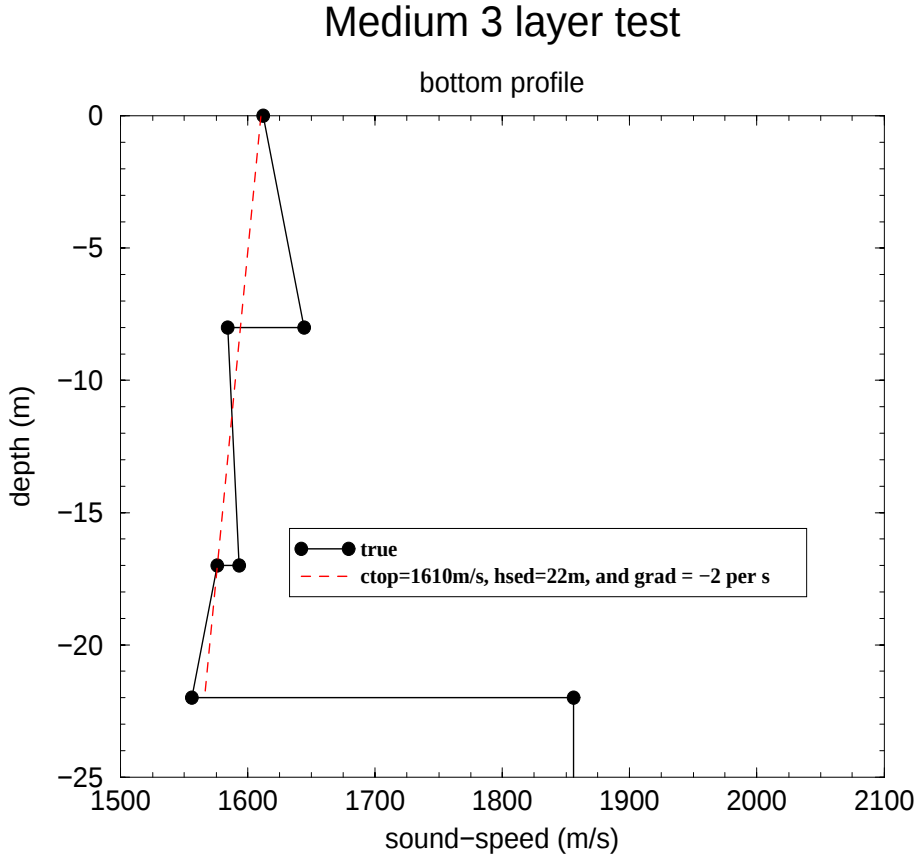
Figure 1: Simulated 3 layer environment assuming the linear sound-speed profiles shown for each sediment layer. The top sediment layer is 8m thick, the next is 9m thick, and the last is 5m thick.
