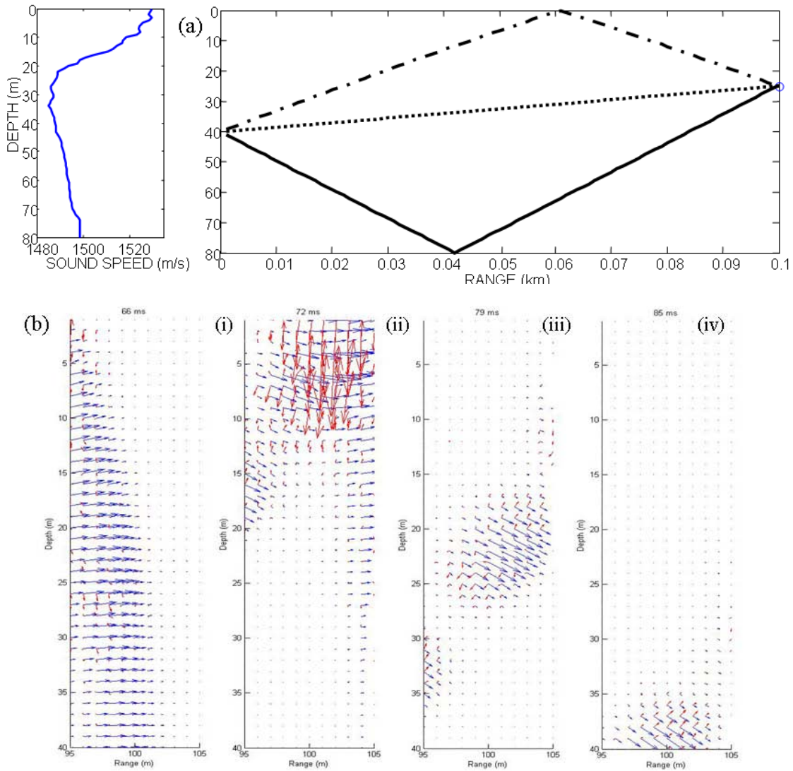
Fig. 3. (a) Rays showing direct path (dotted), surface path (dash-dot) and bottom path (solid) for source at depth 40 m and receiver at depth 25 m. Water sound speed and seabed represent SW06 conditions shown on left. (b) Quiver plots of the complex instantaneous intensity as a function of time for a 1000 Hz signal, bandwidth 300 Hz interacting with a rough sea surface (rms waveheight = 0.17 m), source range 100m. The active intensity is shown in blue and reactive intensity is shown in red (i) The direct path moves forward with little reactive component (ii) Multipath interference forms a vortex in active intensity and a sink or convergence of reactive intensity (iii-iv) further time evolution shows reactive intensity following the pressure gradient of the interference pattern (the reactive intensity has been magnified 10X to emphasize the direction).
