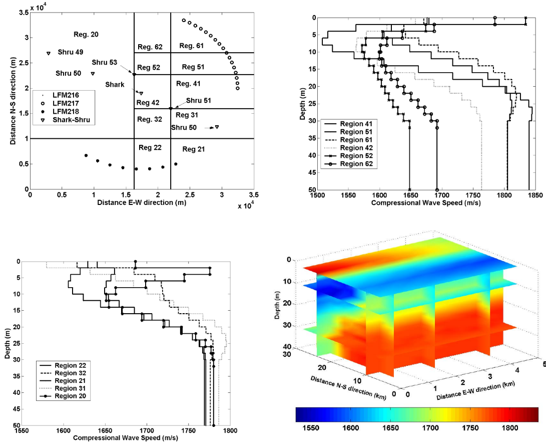
Figure 1. The top left panel shows the eleven regions for which the compressional wave speed profiles were estimated. The figure also shows the location of receiver units and shot location. The shots 13, 14, 15 and 16 on day 217 are in the NE region with shot number increasing from the top. The shots 7 and 8 on day 218 were in the southern region with the shot number increasing from the west. The top right panel shows the compressional wave speed profiles for six regions and the bottom left panel shows the compressional wave speed profiles for the remaining five regions. The bottom right panel shows a 3D representation of the compressional wave speed for a volume representing the region 21, 22, 31, 32, 41, 42, 51, 52, 61 and 62. This was obtained by interpolation of the profiles of the ten regions.
