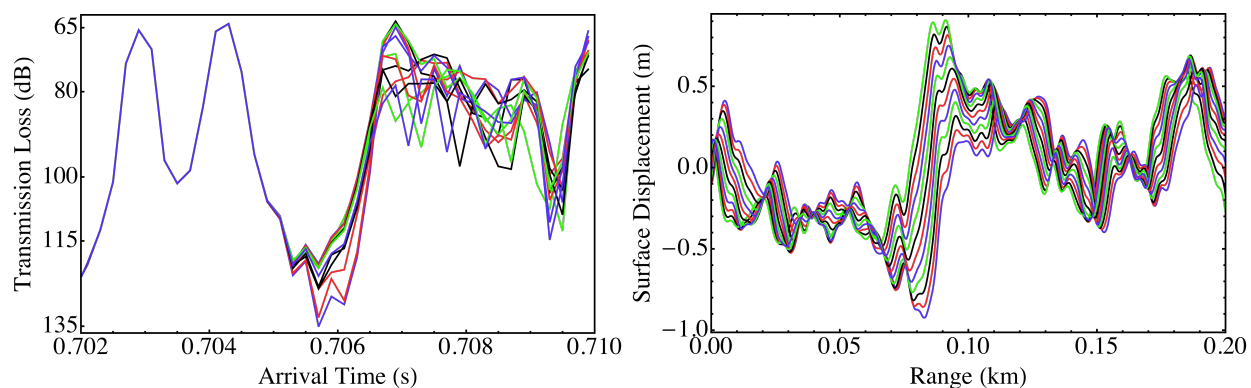
Figure 7: (a) Transmission Loss for rough-surface transmissions with time steps of 0.125 s. (b) Rough surfaces used to generate respective runs shown in 7(a).
