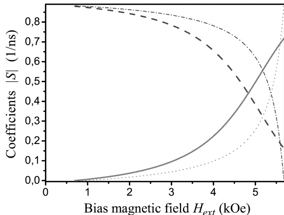
FIG. 8: (color online) The coefficients |S| , which show the amplitude of excitation of coupled spin wave modes by microwave magnetic field, as a function of a bias magnetic field. While calculating we put: L_1/R = 1/10, d/R = 1/25 and \mathbf{h}_\sim = \{0, 0.1kOe, 0\} . Solid and dashed lines: The coefficients |S| for lower mode (quasi-antisymmetric one at small bias external fields) and upper mode (quasi-symmetric one at small bias external fields), respectively, obtained from expression (12c). Dotted and dashed dotted lines: The same coefficients |S| obtained from approximate expressions (16a) and (16b).
