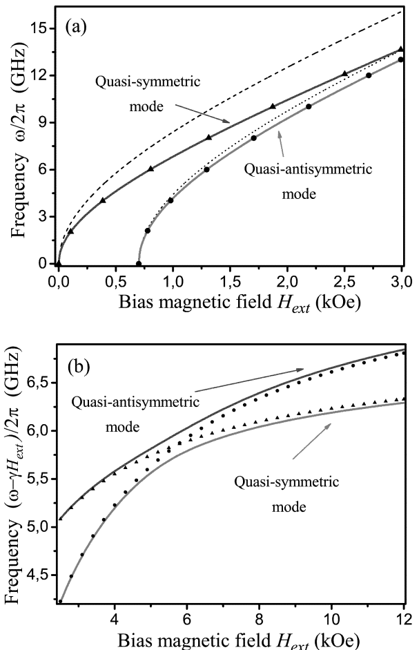
FIG. 3: (color online) (a) The frequencies of linear coupled excitations in a two layer nano-pillar as a function of bias magnetic field. Solid lines : The exact solutions of secular Eq. (9). Triangles and dots : The frequencies \omega_1/2\pi and \omega_2/2\pi respectively (approximate expressions (10)). Dashed and dotted lines : The traditional Kittel expressions for in-plane magnetized ferromagnetic film 13 : \omega_{K,1} = \gamma\sqrt{H_{ext}(H_{ext} + 4\pi M)} and \omega_{K,2} = \gamma\sqrt{(H_{ext} - \tilde{H}_2)(H_{ext} - \tilde{H}_2 + 4\pi M)} respectively. (b) The frequencies (\omega - \gamma H_{ext})/2\pi as a function of bias magnetic field. Solid lines : The exact solutions of secular Eq. (9). Triangles and dots : (\omega_1 - \gamma H_{ext})/2\pi , (\omega_2 - \gamma H_{ext})/2\pi respectively (approximate expressions (10)). While calculating we put: L_1/R = 1/5 , L_2/R = 1/10 , d/R = 1/25 .
