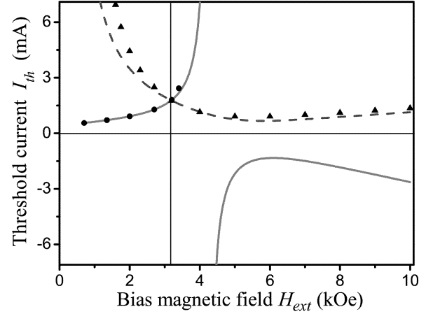
FIG. 6: (color online) The threshold current for excitation of coupled linear spin wave modes represented on Fig. 3 as a function of a bias magnetic field. While calculating we put: L_1/R = 1/5, L_2/R = 1/10, d/R = 1/25, R = 50nm, \alpha = 0.01, \varepsilon_1 = \varepsilon_2 = 1 . Solid and dashed lines: The threshold current for excitation of lower mode (quasi-antisymmetric one at small bias external fields) and upper mode (quasi-symmetric one at small bias external fields), respectively, obtained from approximate Eq. (14). Dots and triangles: The same threshold current obtained from Eq. (13).
