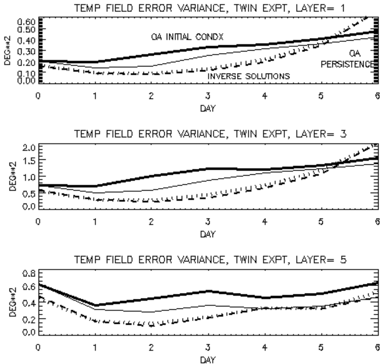
Figure 1. Twin Experiment: Temperature field error variance in the entire data domain for (thin line) persistence of the Initialization Survey OA, (thick line) model run initialized from the Initialization Survey OA, (dotted line) first iteration model run initialized with the inverse solution and (dashed line) second iteration model run initialized with the inverse solution for (top to bottom) layers 1, 3 and 5. Note the differing scales on the abscissas.
