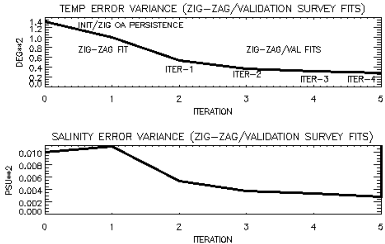
Figure 2. Data from Aug 1993 IFF cruise. (Top) Temperature and (bottom) Salinity error variance of fits of the Zig-Zag and Validation Survey hydrographic data. The first point corresponds to persistence of the Zig-Zag/Initialization Surveys OA. The second point corresponds to the second iteration of the Case 6 model fit using the zig-zag data alone. The third through sixth points correspond to the first through fourth iterations of the Case 8 model fits.
