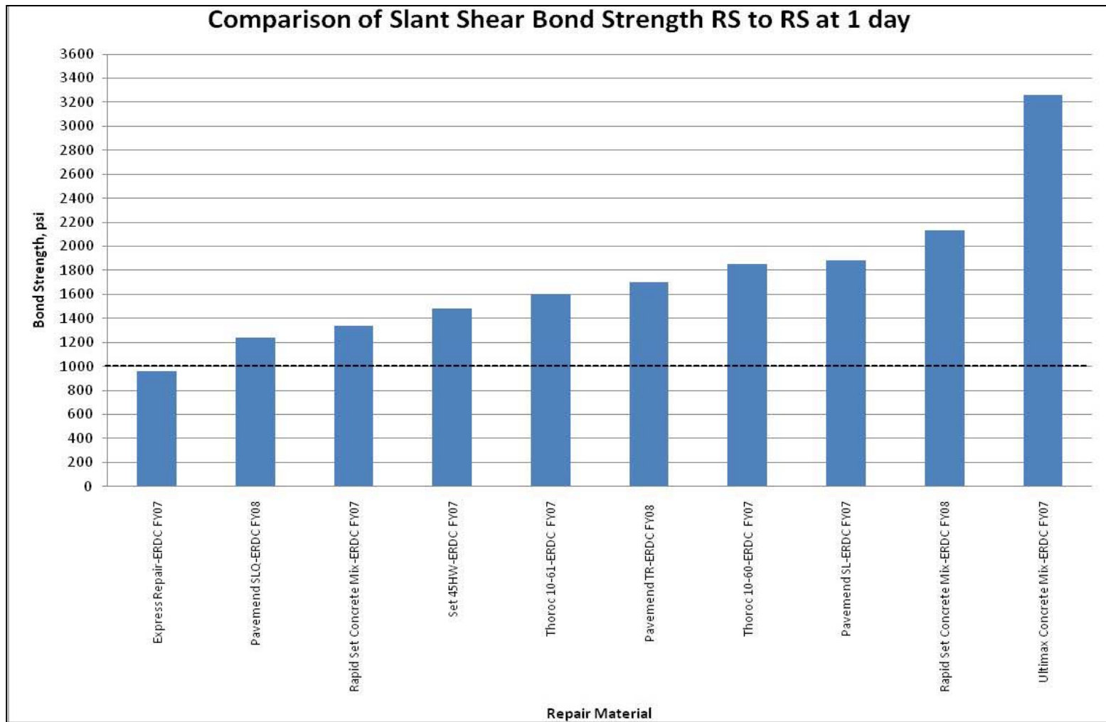
Figure 15. Comparison of product bond strength to self at 1-day cure.
