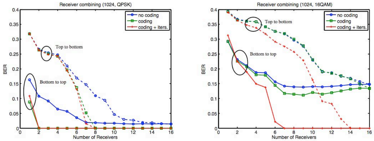
Figure 4. Array performance with receive elements combined sequentially from bottom-to-top and top-to-bottom. (a) QPSK BER vs. number of receive elements combined. (b) 16-QAM BER vs. number of receive elements combined. Bottom of the array is near the seafloor.
