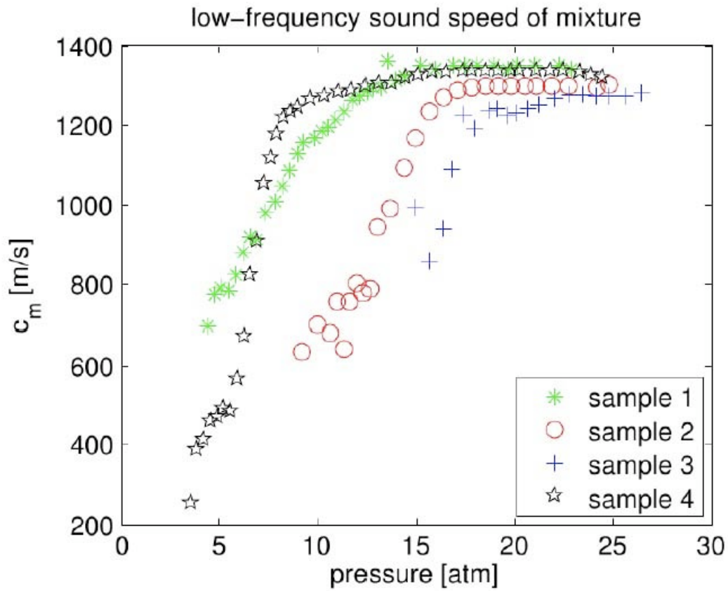
Fig. 5. Measured sound speeds of hydrate mixtures.
