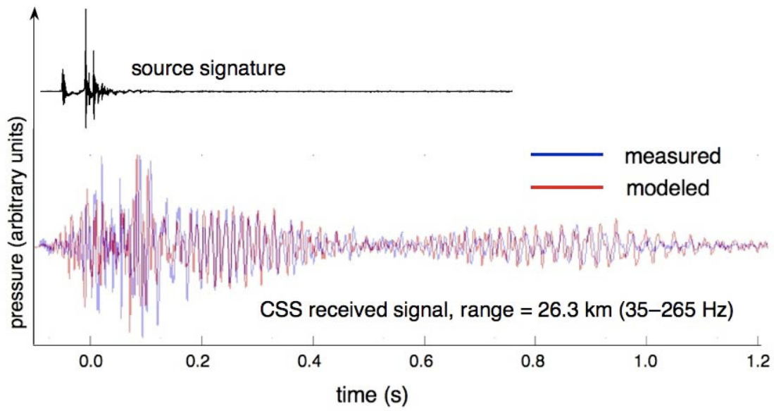
Fig. 6. Broadband propagation modeling from SW06. The upper curve is the CSS Event 26 source signature, deployed at 26 m depth. The lower curves are measured and modeled propagation 26 km downrange from the source.
