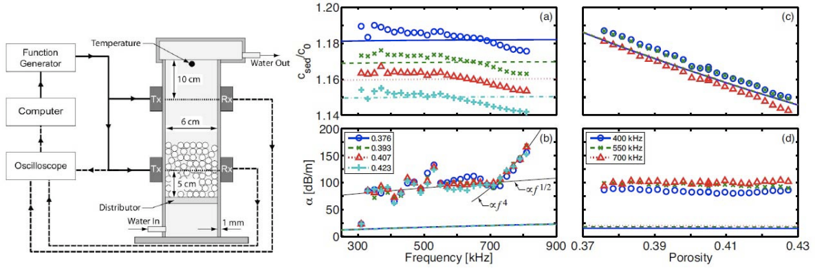
Fig. 2 On the top, a schematic diagram of the porosity control apparatus is shown. Solid (dashed) lines denote the transmitted (received) electrical signal paths. The glass beads are not drawn to scale. Water flowing into the bottom of the column causes motion of the sediment grains, with the resulting porosity after cessation of the flow dependent upon the flow rate. Sound speed and attenuation are measured using the pairs of Rx-Tx transducers. A typical measurement of sound speed (a) and attenuation (b) versus frequency, for various porosities is shown in the middle frame. Sound speed (c) and attenuation (d) versus porosity for three frequencies is shown on the right. The solid lines represent predictions of the effective density fluid model [24]. Biot-like ( f^{1/2} ) behavior is seen below about 700 kHz, but at higher frequencies, the attenuation follows f^4 , which suggests a multiple scattering mechanism. Figure (c) also shows that porosity is a very good indicator of sound speed, while attenuation (d) is independent of porosity.
