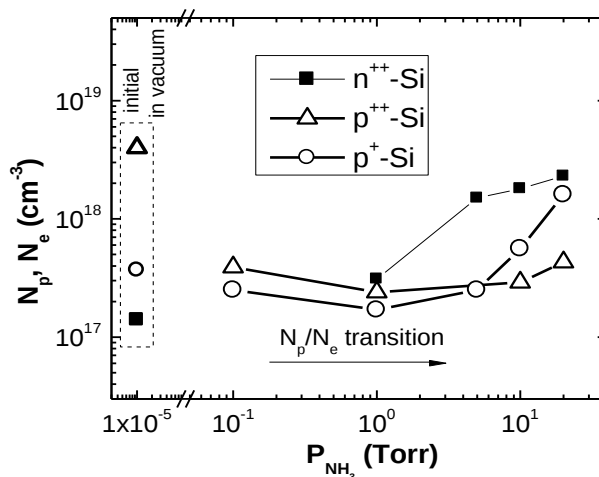
Fig. 2. Dependence of the free carrier concentration in meso-PSi films of different initial conductivity type and doping level vs \text{NH}_3 pressure.
