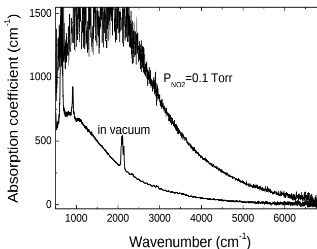
Fig. 1. Absorption spectra of as-prepared p^{++} -PSi films in vacuum or in \text{NO}_2 atmosphere.
