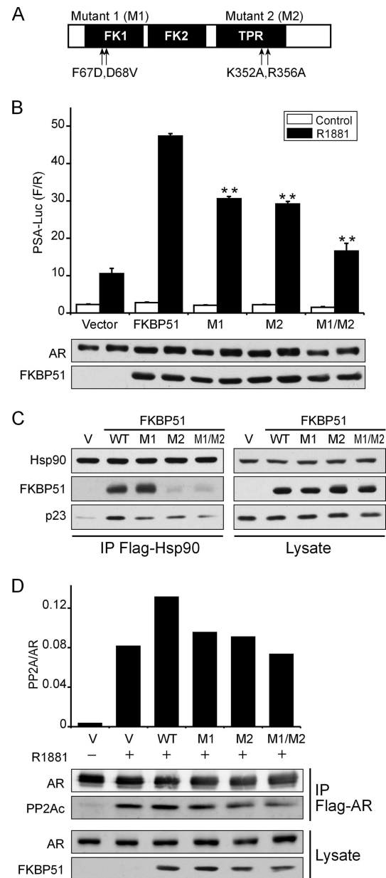
FIG. 8. Point mutations that decrease FKBP51 activity reduce its ability to enhance AR-dependent transcription and superchaperone complex assembly. (A) Diagram of FKBP51 showing the three major structural domains (black shading) and the positions of the point mutations that disrupt prolyl isomerase activity (M1; F67D, D68V) and binding to Hsp90 (M2; K352A, R356A). The M1/M2 form of FKBP51 contains both sets of point mutations. (B) PSA reporter assay with wild-type and mutant forms of FKBP51. Asterisks denote P values (**, P < 0.01 ) comparing the activities of mutant forms of FKBP51 to that of wild-type FKBP51. The mutant forms of FKBP51 show the same reductions in activity relative to wild-type FKBP51 when the data are plotted as fold activation induced by R1881 (not shown). (C) Effects of FKBP51 point mutations on enhancement of superchaperone complex assembly. PC-3 cells were cotransfected with Flag-Hsp90 and untagged forms of FKBP51. Hsp90 complexes were isolated by IP and immunoblotted for chaperones (transfected FKBP51, endogenous p23). (D) Analysis of mutant forms of FKBP51 by using the PP2A-AR to assess the effect on androgen binding to AR. The amount of PP2A that coimmunoprecipitates with AR was plotted as a PP2A/AR ratio. The FKBP51 enhancement of androgen binding to AR obtained with (wild-type protein) was reduced in the M1, M2, and M1/M2 mutant forms of FKBP51. V, vector.
