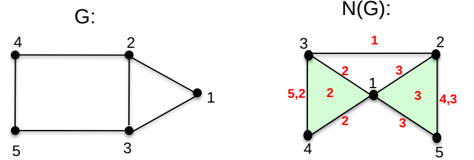
Fig. 3. A graph (G) and its labeled neighborhood complex \mathcal{N}(G)
