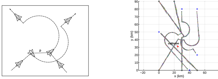
Fig. 5. The modes of operation for the aircraft collision avoidance example (left). Testing the aircrafts with v = 0.3 \text{ km/sec} , \omega = 0.03 \text{ rad/sec} , and p = [4.5, 5.5] \text{ km} under bounded disturbances \|u\| \leq 0.03 \text{ km/sec} (right). We define the collision distance as 1 \text{ km} . Circles represent initial positions and rectangles are goal positions. A collision is discovered after exploring about 8,600 nodes with p = 5.25 \text{ km} .
