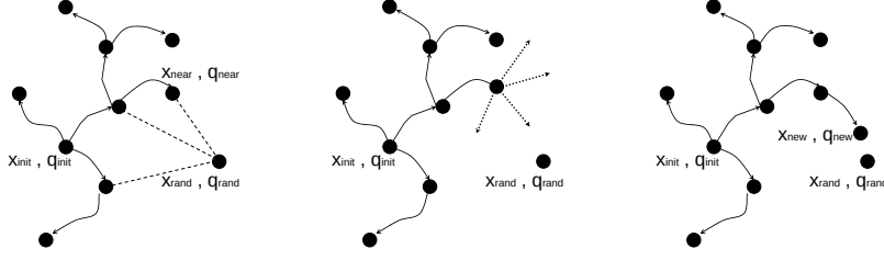
Fig. 1. The Testing algorithm (inspired by the RRT [19]). The test set is represented as a tree T with nodes as states (x, q) and edges as inputs u \in \bar{U} . First a new state is generated at random, x_{rand}, q_{rand} . The algorithm then determines the closest state, x_{near}, q_{near} in the tree to the random state ( left ). It determines which u \in \bar{U} brings x_{near}, q_{near} closest to x_{rand}, q_{rand} ( center ). u_{new} is applied for a duration \delta t and the new node x_{new}, q_{new} and edge u_{new} are added to the tree ( right ).
