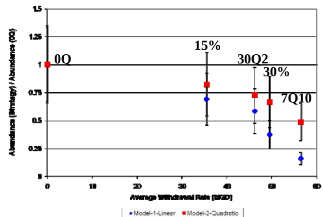
Figure 4: Normalized abundance (SD) of darters and average withdrawal rate for each flow management scenario.
