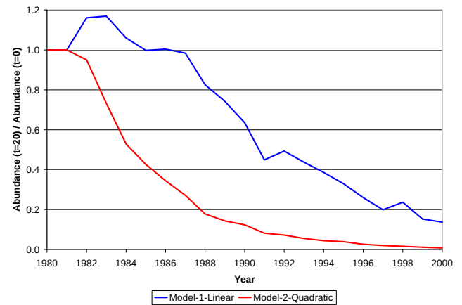
Figure 3: Normalized abundance predictions of two survival models for the null withdrawal strategy.
