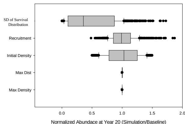
Figure 5: Sensitivity analysis assessing the relative influence of each demographic component to Year-20 darter abundance (linear survival model only).
