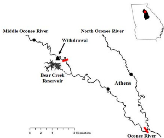
Figure 1: Middle Oconee River study reach within the Upper Oconee River Basin (inset) with reach boundaries (red), location of the pump-storage reservoir intake (triangle) and USGS gages (black).
