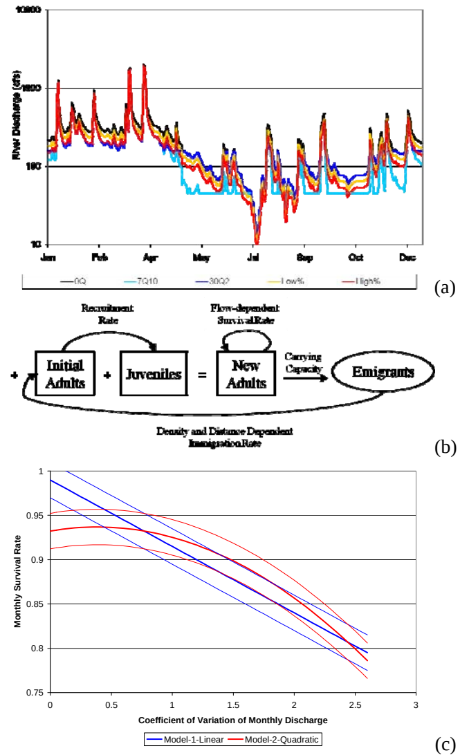
Figure 2: Effects of flow management strategies in a typical flow year, conceptual representation of the population model, and survival model uncertainty.
