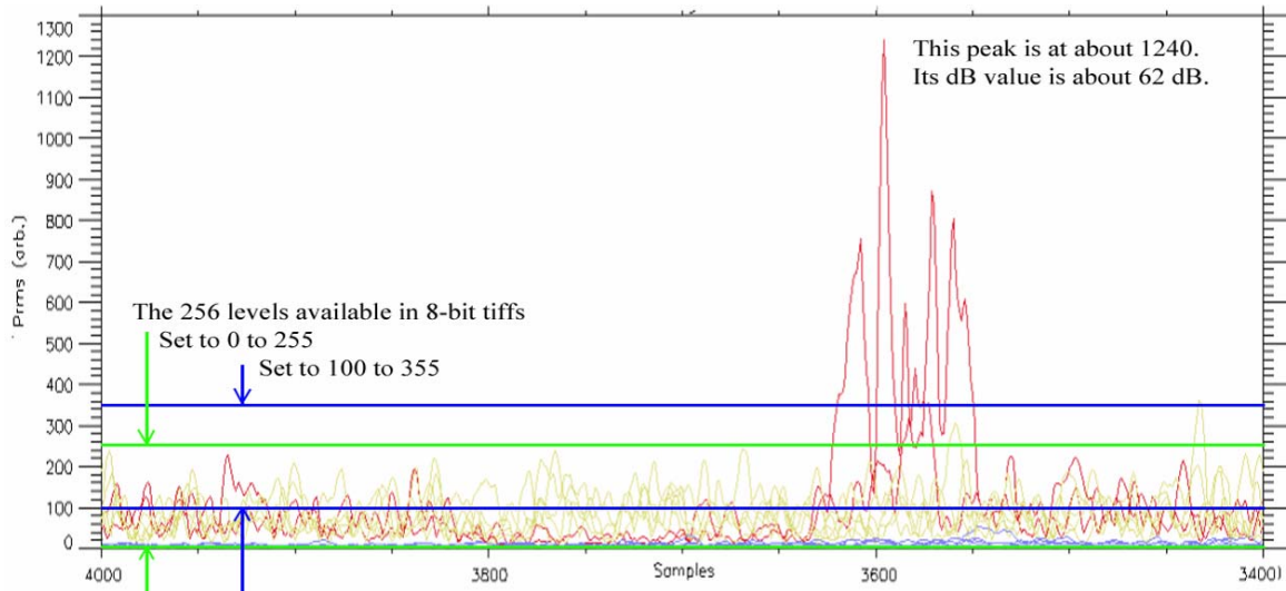
Figure 2: This is a plot of the 12-bit digital data taken with the quantitative side-scan sonar (same hardware and set of pings that produced Fig. 1). However, the output from the towfish was sent to a separate digitizer. Note that it took 1240 levels of the available 4096 ( 2^{12} ) levels to capture the peak (versus the 256 levels that can be extracted from the 8-bit tiffs). Again the yellow lines represent the background clutter levels and the red represents the target, as well as, the target-shadow levels. The light blue data lines are separately measured background noise (no pinging) faintly seen just above the zero level. The heavy, horizontal blue and green lines simulate a priori settings of the knobs from 100 to 355 and 0 to 255, respectively. Clearly the 12-bit data capture what will generally be the full dynamic range of the side-scan data without a priori selection of settings. If one ever thought the 12-bit data would have limitations in the real world, they might select to use 16-bit data with 65536 levels and 96 dB dynamic range.
