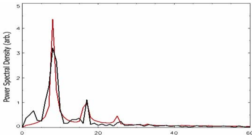
Figure 4: The average Fourier transform of the backscatter data at 150 and 300 kHz (black) and the Fourier transform of the simulated backscatter from the modeled sinusoidal profile (red).
