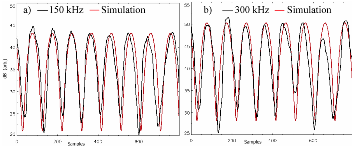
Figure 4: The diagrams show the backscatter from 150 kHz and 300 kHz, respectively. In red is a single simulation for both based on computed Lambert backscatter from a model sinusoidal profile calculated by the technique given in ref. [1]. The maxima are scattering from the front facing slopes and the minima are from the back slopes.
