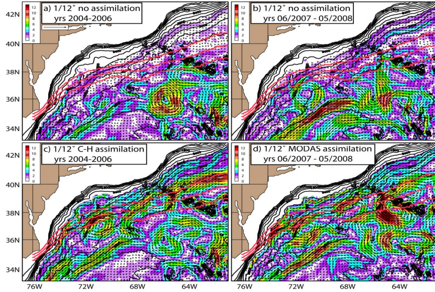
Figure 7. Mean depth averaged velocities in layers 27 to 29 (~3500-4500 m) four 1/12^\circ global HYCOM simulations: (a) interannually forced weak Gulf Stream with separation velocity of 1.1 \text{ m s}^{-1} ; (b) interannually forced stronger Gulf Stream with separation velocity of 1.4 \text{ m s}^{-1} ; (c) Cooper-Haines data assimilation twin of the weak Gulf Stream and (d) MODAS synthetic temperature and salinity profile data assimilation twin of the stronger Gulf Stream.
