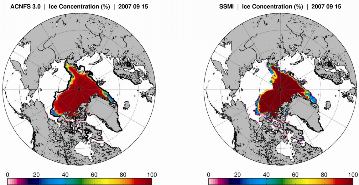
Figure 1. Ice Concentration (in percent) from a) ACNFS and b) SSM/I. Images valid for 15 September 2007. The black line is an independent ice edge from the NIC.
