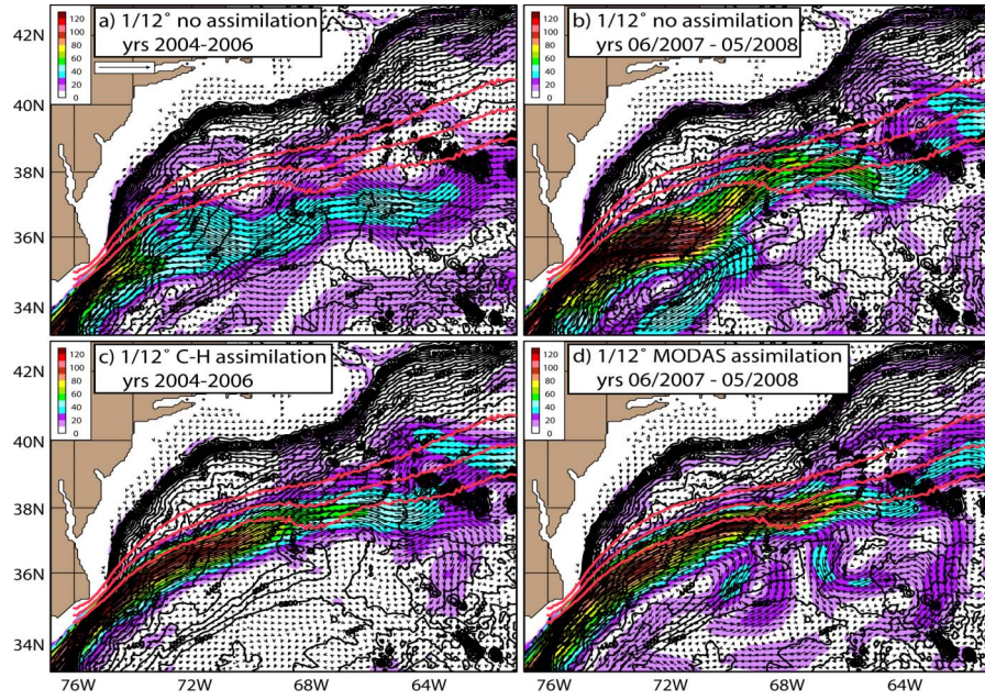
Figure 6. Mean velocities in layer 6 (~25 m) with the mean Gulf Stream pathway \pm 1\sigma overlaid in red and the bathymetry contoured at 200 m intervals from four 1/12^\circ global HYCOM simulations: (a) interannually forced weak Gulf Stream with separation velocity of 1.1 \text{ m s}^{-1} ; (b) interannually forced stronger Gulf Stream with separation velocity of 1.4 \text{ m s}^{-1} ; (c) Cooper-Haines data assimilation twin of the weak Gulf Stream and (d) MODAS synthetic temperature and salinity profile data assimilation twin of the stronger Gulf Stream.
