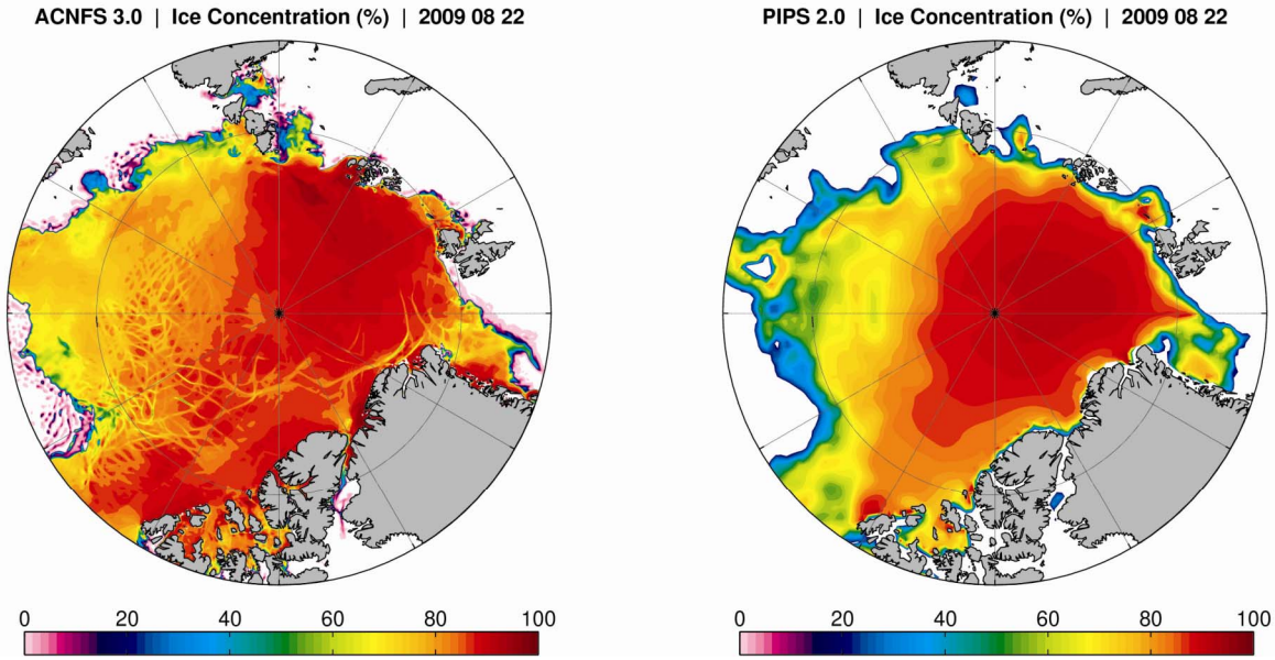
Figure 3. Ice concentration (%) from a) ACNFS and b) PIPS 2.0. Valid August 22, 2009. Areas of lower concentration can be seen just north of Greenland in ACNFS (a) but not in PIPS 2.0 (b).
