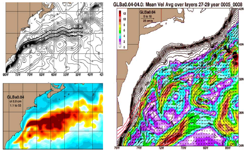
Figure 5. Climatologically forced 1/25° simulation with the mean SSH and mean observed GS pathway in upper left and SSH standard deviation in lower left and layer 27-29 (~3500-4500 m) currents in right panel.
