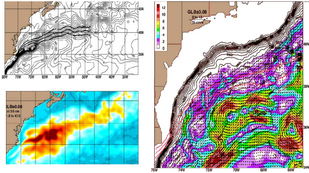
Figure 4. Climatologically forced 1/12° simulation with the mean SSH and mean observed GS pathway in upper left and SSH standard deviation in lower left and layer 27-29 (~3500-4500 m) currents in right panel
