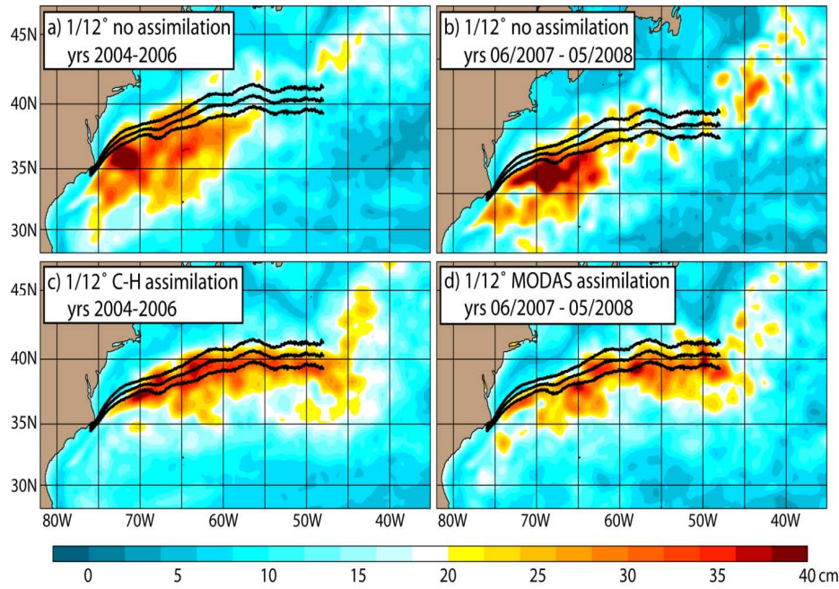
Figure 8. Standard deviation of the sea surface height for four 1/12° global HYCOM simulations: (a) interannually forced weak Gulf Stream with separation velocity of 1.1 \text{ m s}^{-1} ; (b) interannually forced stronger Gulf Stream with separation velocity of 1.4 \text{ m s}^{-1} ; (c) Cooper-Haines data assimilation twin of the weak Gulf Stream and (d) MODAS synthetic temperature and salinity profile data assimilation twin of the stronger Gulf Stream.
