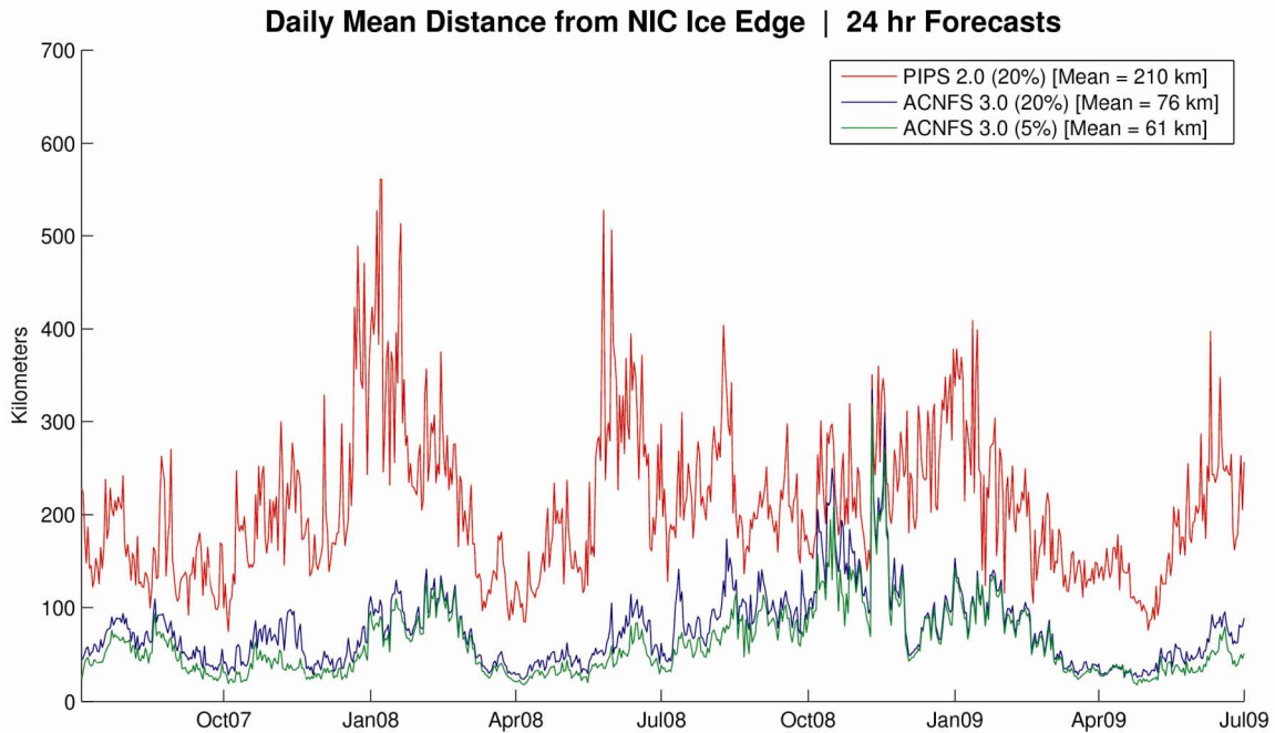
Figure 2. Daily mean distances (km) from the NIC observed ice edge locations to the ice edge locations using the 24 hr forecasts from ACNFS (20%-blue Mean=76km and 5%-green Mean=61km) and PIPS 2.0 (20%-red Mean=210km) for July 2007- June 2009.
