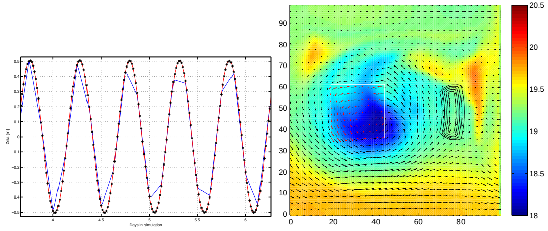
Figure 1: (left) Barotropic tide solution using harmonics (blue cross) versus boundary nesting (blue line) and truth (black). (right) Temperature solution (shown in ^{\circ}\text{C} ) of internal tide in both the parent and child nests of the model. A large, mesoscale eddy is shown interacting with the internal tides.
