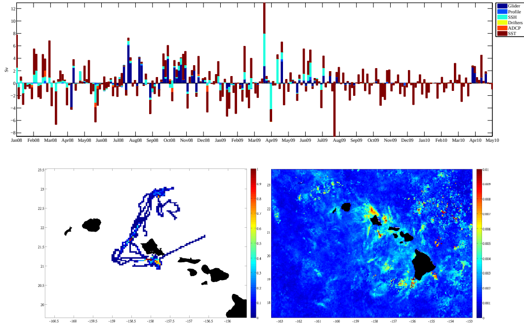
Figure 3: (top) Time-series showing the total contribution of each observation type to the transport increment made in the assimilation (e.g., a bar of 2Sv, shows that during the 4-day window, the transport was changed by 2 Sv, and the breakdown of colors illustrate the contribution of each type). (bottom, left) The RMS of the contributions from the SeaGlider over all assimilation windows as compared with (bottom, right) the contribution from the SST. The SeaGlider contributes (on average) over 3 magnitude more information on transport than the SST even though the total number of SeaGlider observations are dwarfed by the SST.
