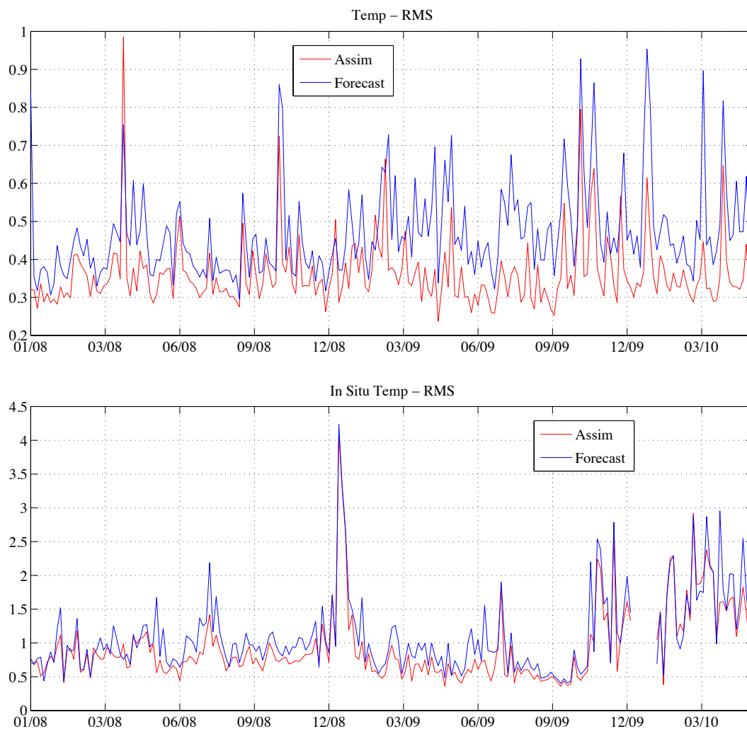
Figure 2: (top) Time-Series of RMS between model and SST observations for the prediction and assimilation cycles. (bottom) Time-Series of RMS between model and in situ observations for the prediction and assimilation cycles.
