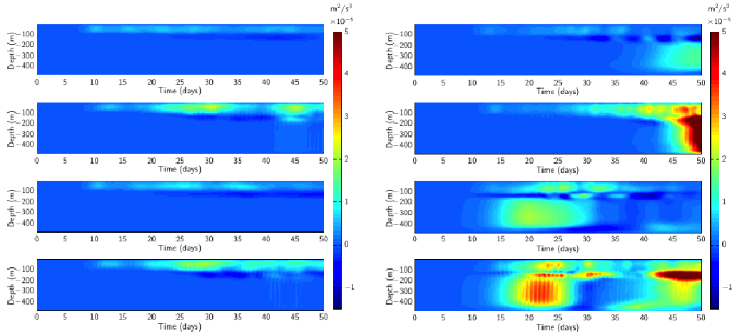
Figure 1 (Left Panel) Hovmuller plot of horizontally averaged vertical buoyancy flux w'b' for four simulations WITHOUT any baroclinicity below the mixed layer. The top panel shows the development due to mixed layer eddies in the top 100m, the second panel shows the influence of wind (no mesoscale meanders), the third shows the effect of an initial mesoscale meander (no wind), and the final panel shows fluxes in presence of both meander and wind. The panel on the right shows the averaged vertically buoyancy flux for simulations WITH the baroclinicity below the mixed layer.
