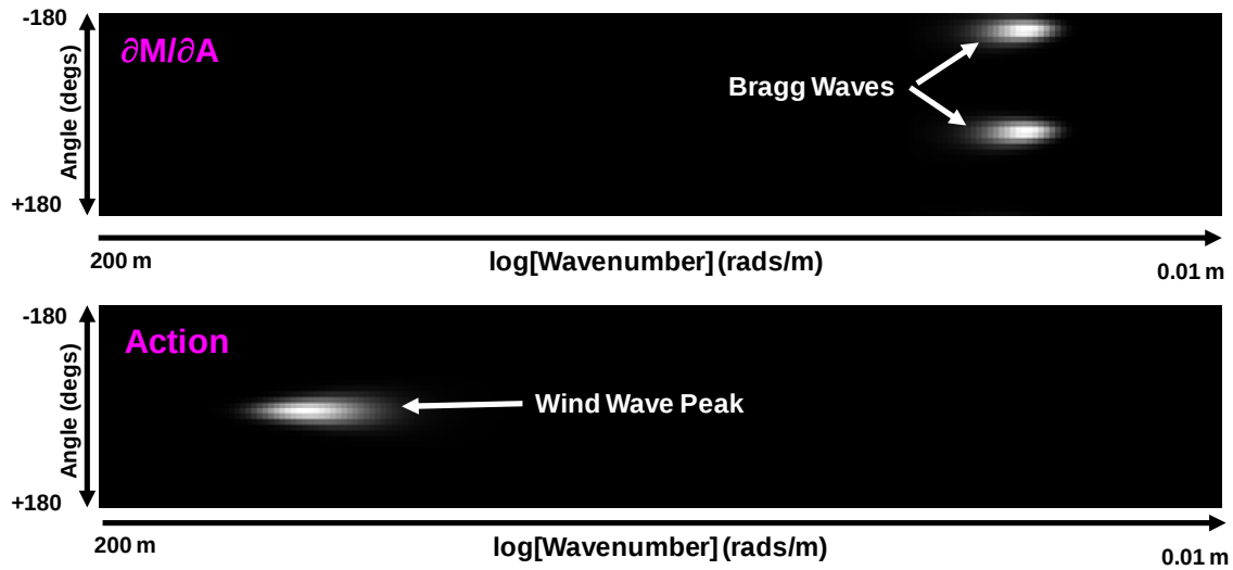
Figure 1: Top image show \partial M/\partial A which is a measure for how much a change in one spectral location will change the model output. This term is dominated by the region around the Bragg wave (bright blobs in the top image) since the model is dominated by Bragg scattering. Note that if we only used Bragg scattering, the top image would be two dots. Bottom image shows the action (i.e. the wave spectrum) which is dominated by the wind wave peaks. Thus this spectral regions dominates the changes in the model due to changes in the integral measures of the wave spectrum.
