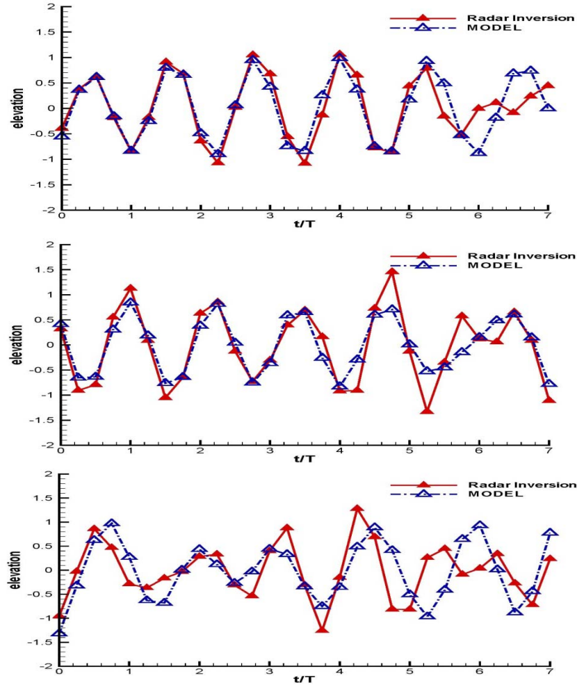
Figure 3: Comparison of the time series of wave elevation at locates A (top panel), B (middle panel), C (bottom panel) between the model prediction (blue line) and radar inversion data (red line). ( T = 6 s).
