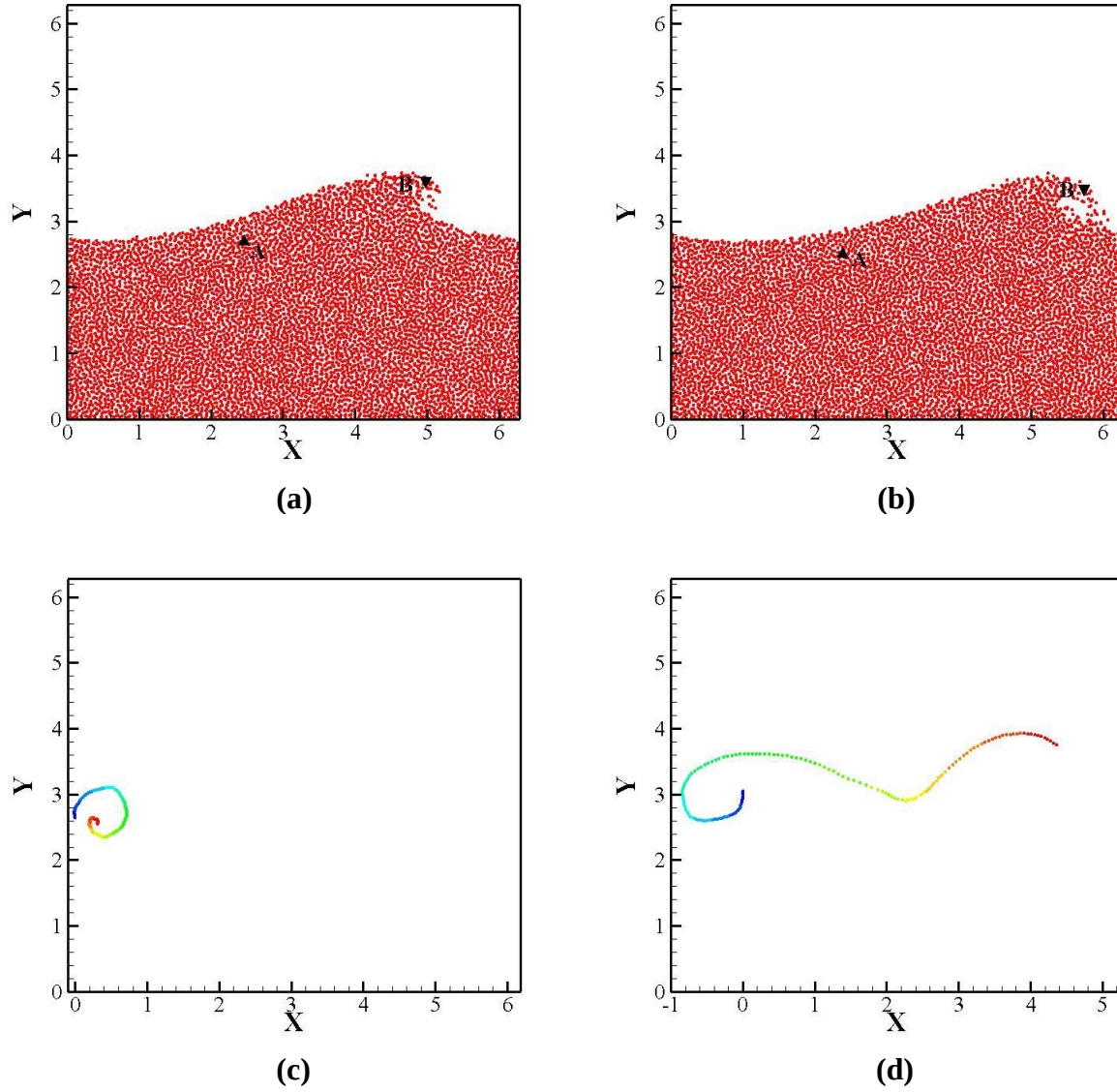
Figure 3. SPH simulation of a two dimensional breaking wave: (a) and (b), snapshots of the breaking wave at two instances; (c) trajectory of particle A; (d) trajectory of particle B. In (c) and (d), initial coordinates of A and B are reset to (0,0); the color on the trajectory indicates time, with blue and red representing the early and later time, respectively.
