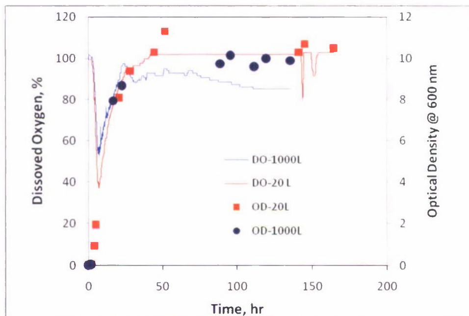
Figure 9. DO and OD Profiles for the 20- and 1000-L Fermentation Runs of Btk. By focusing on the portion of DO responses in 20- and 1000-L fermentation runs, where there were significant metabolic oxygen demand (i.e., up to EFT = 28 hr). Eq. 8 was used to estimate the amount of accumulated O_2 uptake by Btk cultures for 20- and 1000-L fermentation runs up to EFT = 28 hr (Figure 10).
