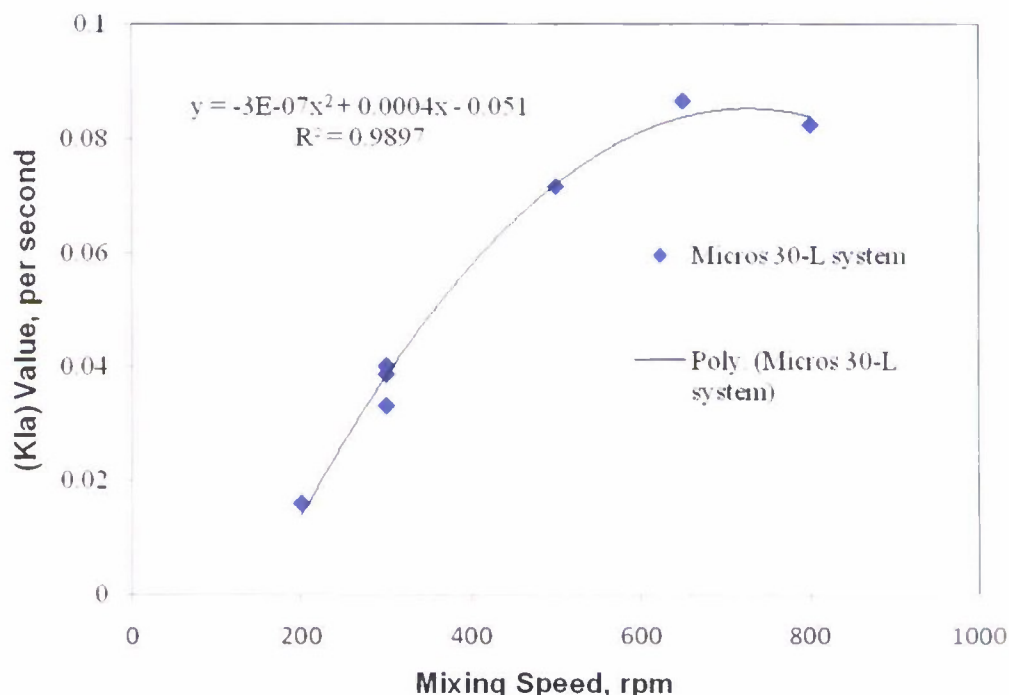
Figure 5. Combined ( k_La' ) Values as Function of Mixing Speeds at Constant 20 slpm and 1 psi.
