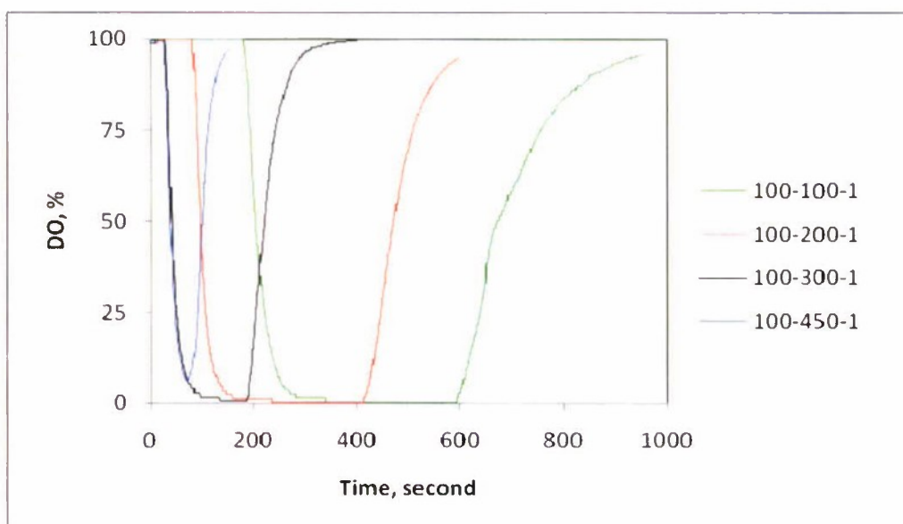
Figure 6. Time-dependent DO Profiles for the 100-L Fermentor System at Different Mixing Speeds (airflow rate and overhead pressure were held constant at 100 slpm and 1 psi, respectively).
