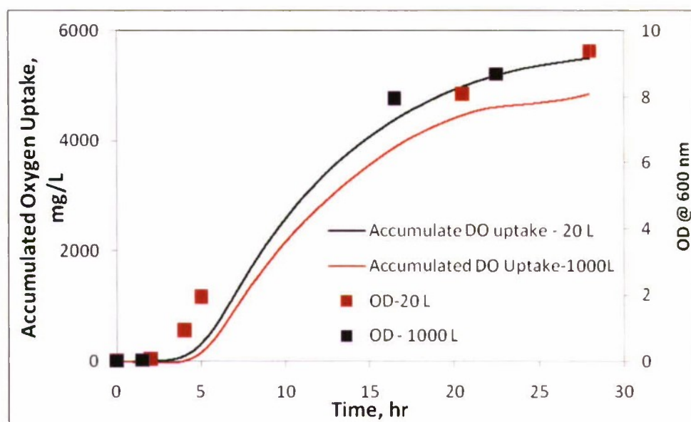
Figure 10. Accumulated DO Uptake Patterns between the 20- and 1000-L Fermentation Runs of Btk.
