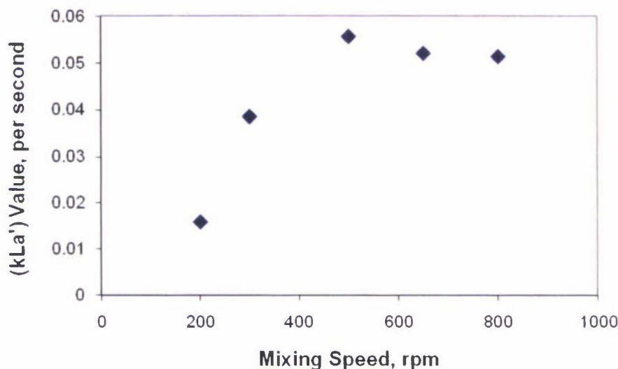
Figure 3. (k_La') Values as a Function of Mixing Speed at Constant 20 slpm and 1 psi.
