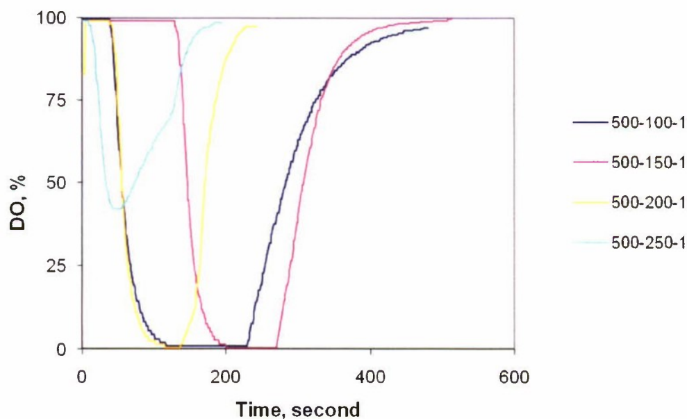
Figure 7. Time-dependent DO Profiles for the 1000-L Fermentor System at Different Mixing Speeds (airflow rate and overhead pressure were held constant at 500 slpm and 1 psi).
