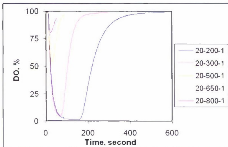
Figure 1. Time-dependent DO Profiles for the 20-L Fermentor System at Different Mixing Speeds (Airflow rate and overhead pressure were held constant at 20 slpm and 1 psi, respectively).
