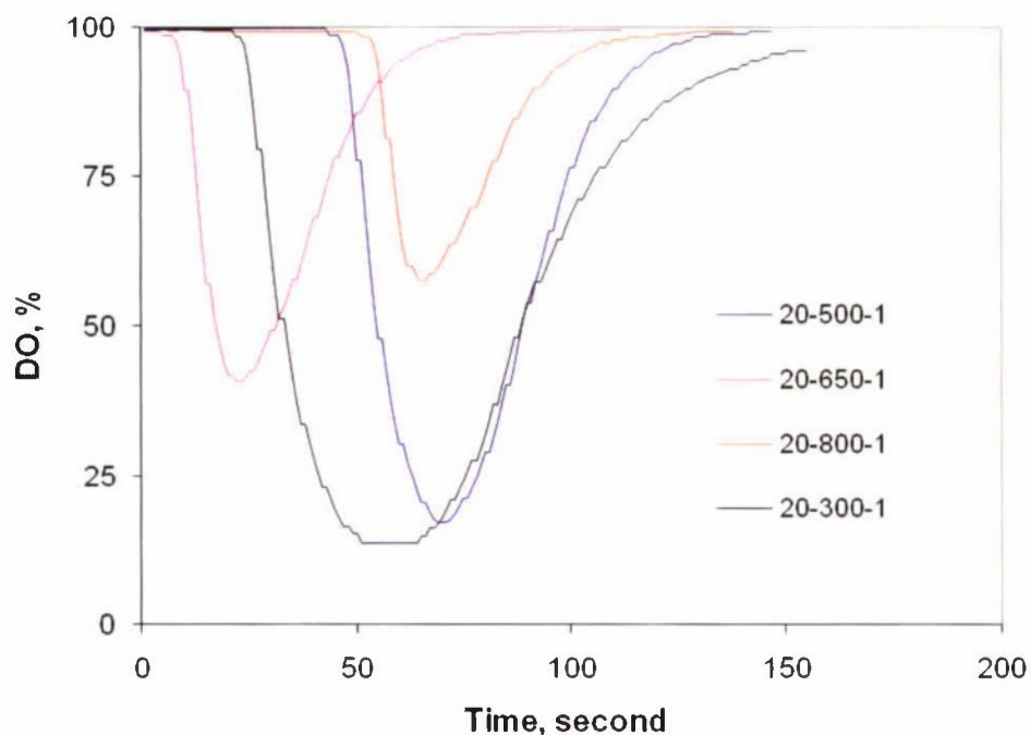
Figure 4. Time-dependent DO Profiles for the 20-L Fermentor System at Different Mixing Speeds without the Overlay Airflow.
