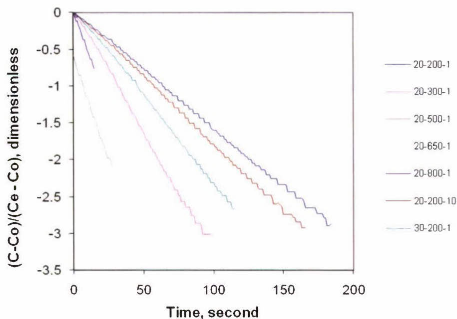
Figure 2. Dimensionless DO Concentration vs. Time for the 20-L Fermentor System.
