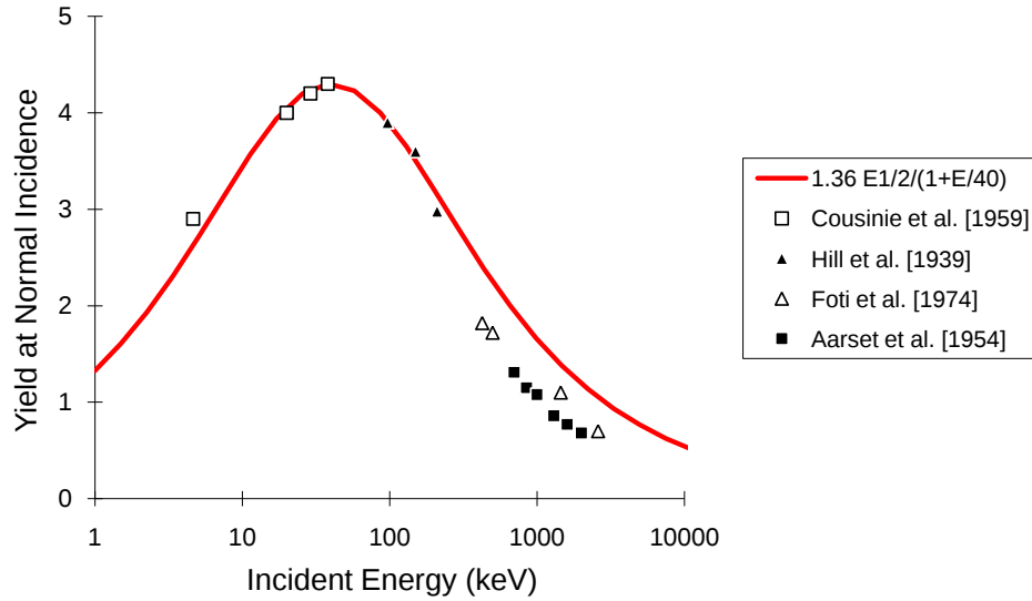
Figure 6. Secondary Electron Emission by Aluminum for Proton Impact at Normal Incidence; Experimental Points as Indicated in the References [17, 18, 19, 20]
