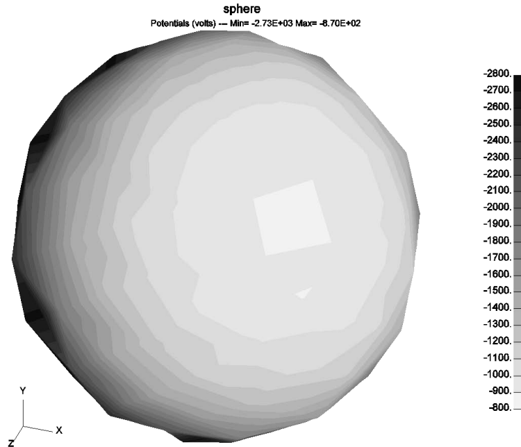
Figure 14. Potentials on Sunlit PATRAN Sphere in Space Viewed from Direction (1,2,3)
