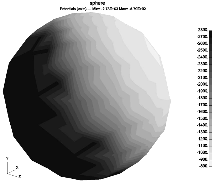
Figure 16. Potentials on Sunlit PATRAN Sphere in Space
