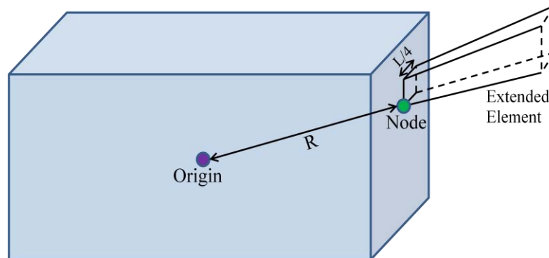
Figure 19. An Extended Element with Analytically Extrapolated Potential Is Appended to Each Boundary Quarter-Square to Implement Non-Zero (Monopole) Potential Boundary Conditions
