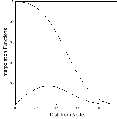
Figure 18. Interpolation Functions F_0 and G_0
