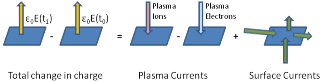
Figure 22. The Change in Charge on a Surface Element Is Made Up of Plasma Currents and Surface Currents
