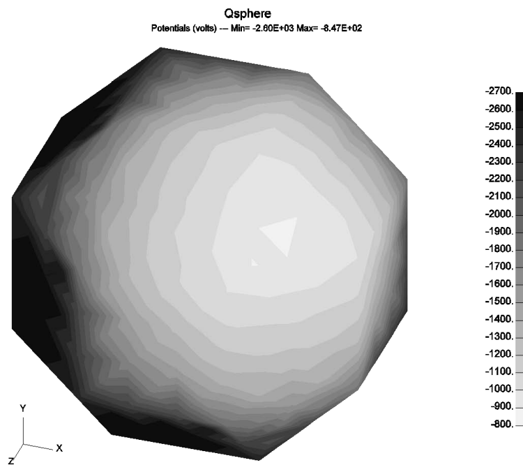
Figure 15. Potentials on Sunlit Qsphere in Space Viewed from Direction (1,2,3)
