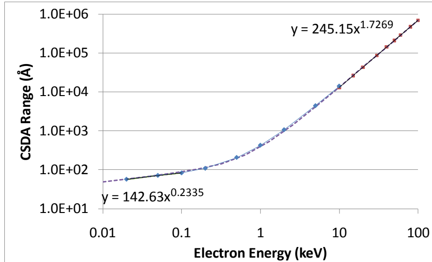
Figure 5. CSDA Range for Electrons in Aluminum. Low Energy Values (Blue Diamonds) From Ashley et al. (Reference 14). High Energy Values (Red Squares) From NIST ESTAR* Database. Dashed Line Is Biexponential Fit.
