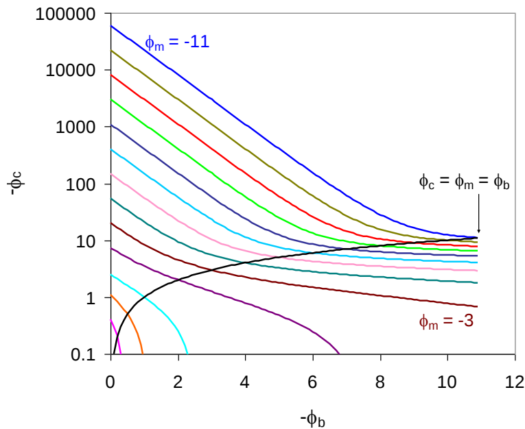
Figure 21. Plot of the Space Charge Cutoff Potential, \Phi_c , Versus Barometric Potential ( \Phi_b = \ln N_i ) for a Series of \Phi_m Values (-0.2, -0.5, -1.0, -2.0, -3.0, -4.0 ... -11.0) – the Point at Which \Phi_m = \Phi_b = \Phi_c Is Also Indicated
