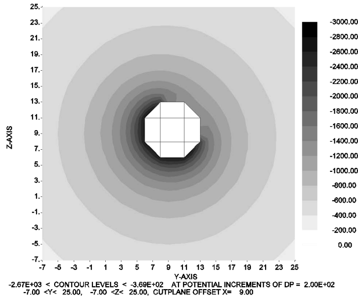
Figure 13. Potentials About Sunlit Qsphere in Space as Computed by NASCAP/GEO
