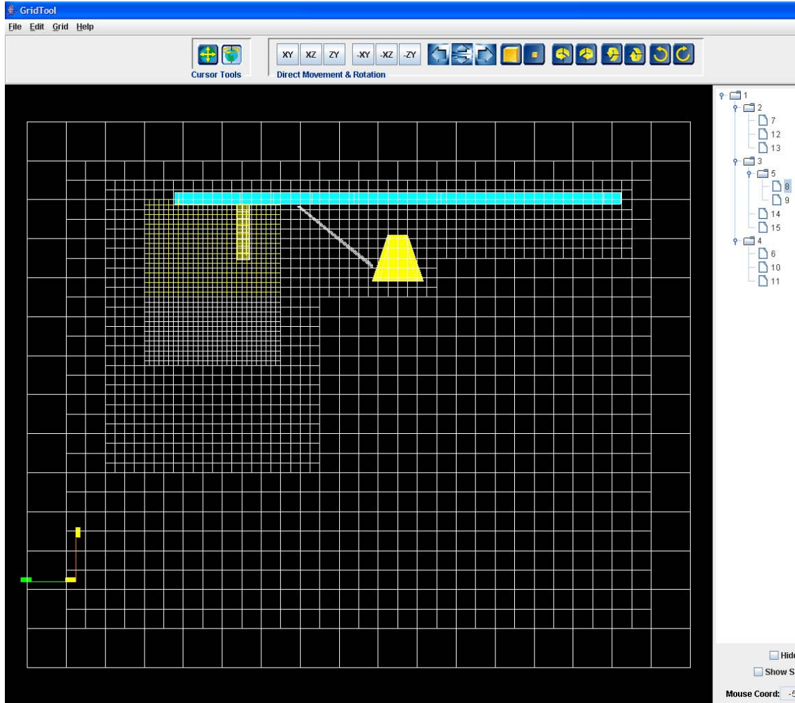
Figure 17. Computational Grid with Subdivision
