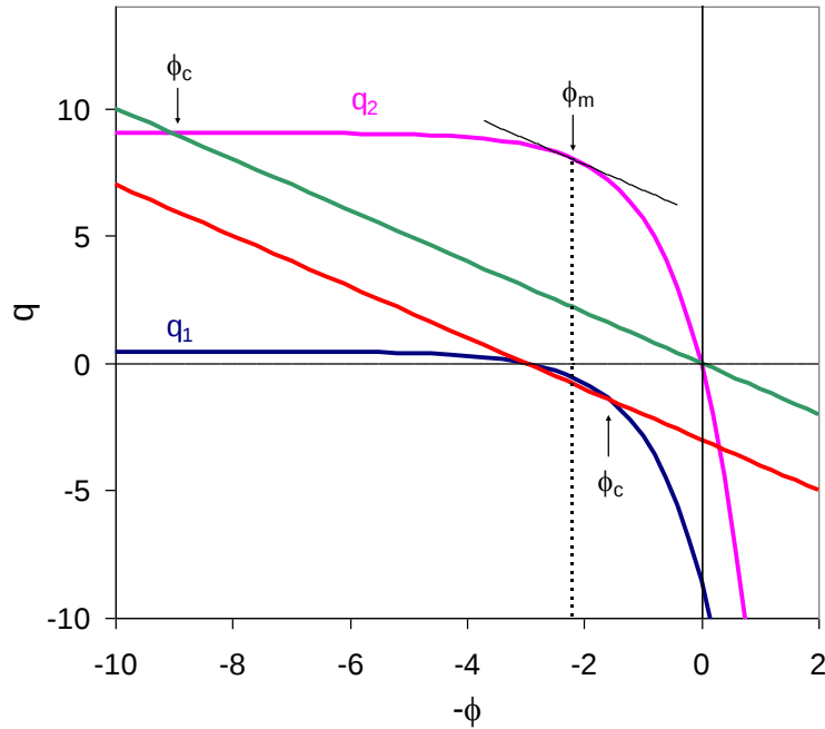
Figure 20. Plots of Space Charge (Curves Q_1 and Q_2 ) as a Function of Potential as Given by Equation 135. The Straight Lines Represent the Maximum Allowable Charge for Non-Oscillatory Potentials. The “Natural” Space Charge, Q_1 or Q_2 Is Acceptable for Which Slopes of the Curves and the Corresponding Line Are Equal.
