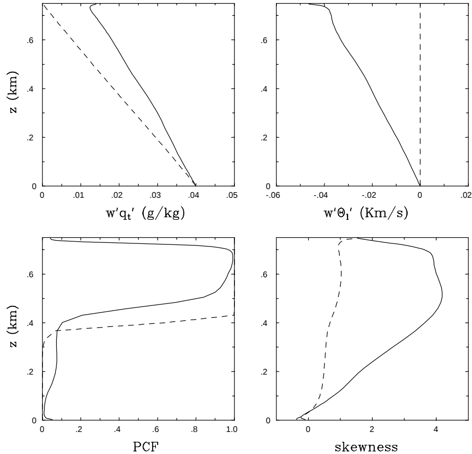
Figure 1. Hour averaged mean vertical profiles for a sample boundary layer driven by surface latent heat flux both with (——) and without (-----) entrained heat and moisture fluxes at the top of the layer. Profiles are total water flux, liquid potential temperature flux, partial cloud fraction, and vertical velocity skewness.
