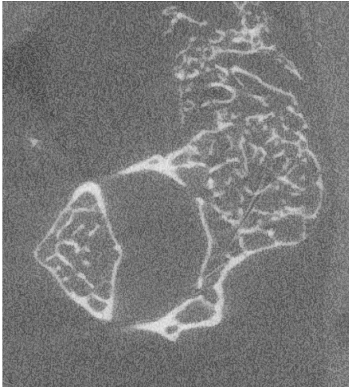
Figure 24: Cross sectional view by microCT imaging of a spine taken 6 weeks after injection of our gene therapy system into the paraspinous musculature.
