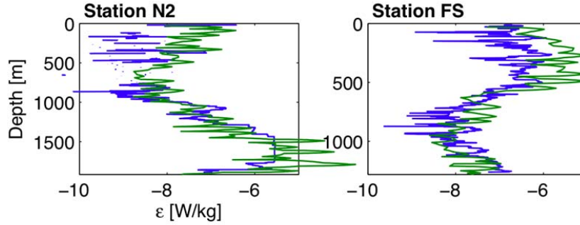
Figure 2: TKE dissipation rate from from LADCP/chipods (green) and Thorpe analyses (blue) at two of the most energetic stations observed during the Luzon Strait pilot. These represent the first direct measurements of abyssal turbulence from shipboard CTD/LADCP.
