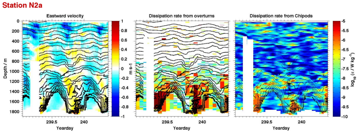
Figure 3: Timeseries of velocity (left) and TKE dissipation from Thorpe overturns (middle) and from \chi (right) for the first occupation of station N2. This was one of the more energetic stations, with vertical displacements and overturns exceeding 500 m, as illustrated by density contours (black).
