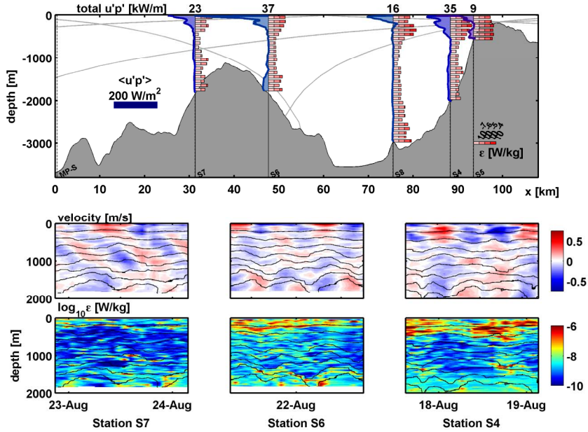
Figure 4: Summary of energy flux and TKE dissipation across the southern line, computed from five 36-h \chi pod/LADCP stations during the 2010 IWISE pilot. These show intense dissipation at the generation site (S4, right), which decays with distance from the ridge (S6 & S7).
