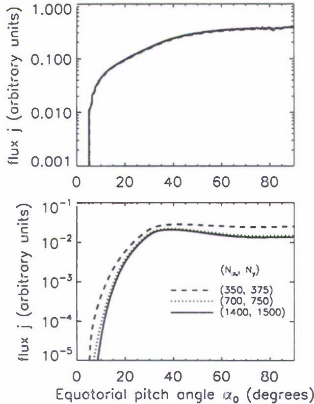
Figure 1. Fluxes for (top) E = 0.5 MeV and (bottom) E = 2.0 MeV at t = 2 d with different choices of N_{\alpha 0} and N_{\beta} using Horne et al. [2005] chorus wave model. In the top plot the three lines are very close together, in contrast to the larger separations shown in the bottom plot.
