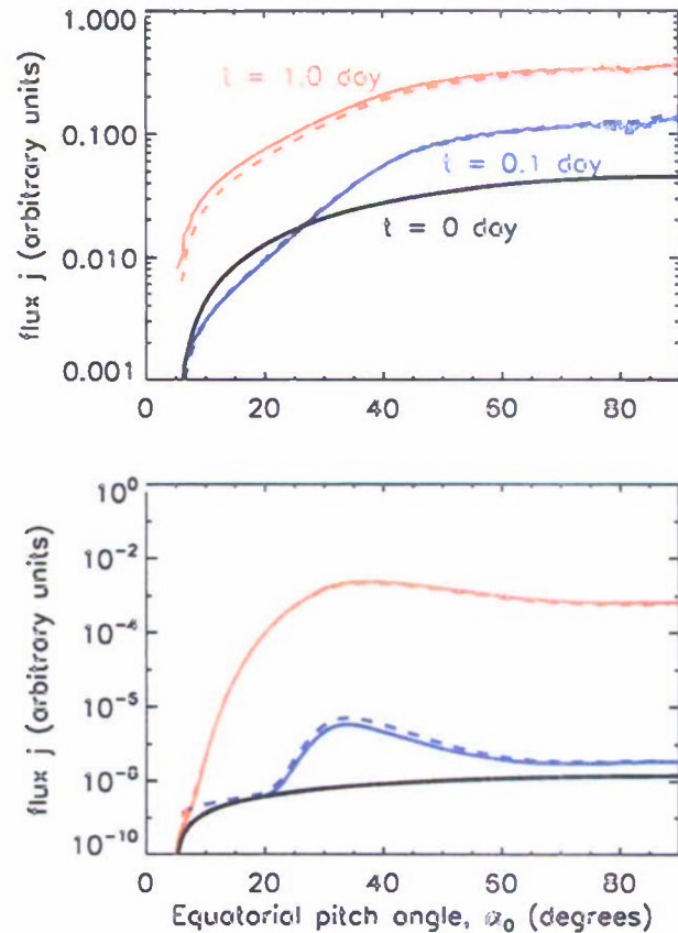
Figure 2. Comparisons between results obtained from the layer method (solid lines) and the Albert and Young [2005] method (dashed lines) for (top) E = 0.5 MeV and (bottom) E = 2.0 MeV at t = 0.1 day (blue lines) and t = 1.0 day (red lines). Here black lines show the initial condition.
