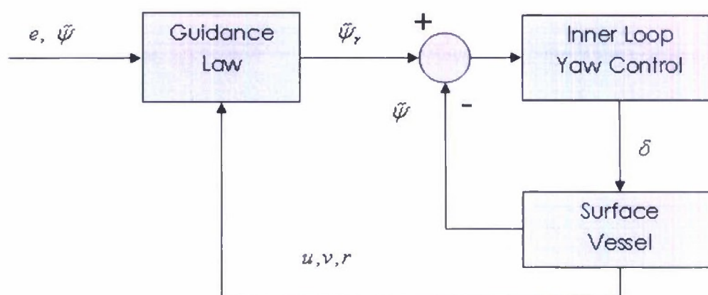
Figure 13: A hierarchical control scheme that mimics good helmsman's behavior. \tilde{\psi} , e are the heading angle and tracking errors respectively; \psi , \psi_r are the actual and reference heading respectively, and \delta is the rudder angle.
