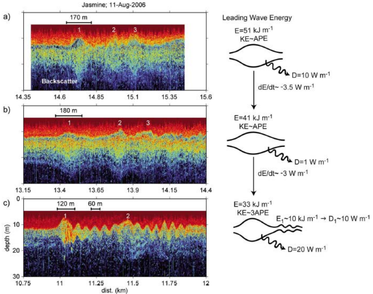
Figure 2 - left) Acoustic backscatter series for the (a) first, (b) second, and (c) third profiling series through Wave Jasmine. Waves propagate to left. Distances are corrected for Doppler shift using ship velocity. (right) Schematic detailing lead wave energetics (Shroyer et al, 2010a).
