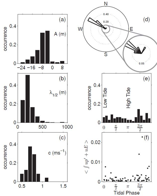
Figure 1 – Histograms of (a) displacement amplitude, (b) half-width, (c) average shoreward wave speed, (d) wave heading, (e) wave arrival time at SW30 relative to the local barotropic tidal height, and (f) average energy flux as a function of tidal phase (low tide corresponds to zero). Panels a-d were calculated from shipboard data; panels e-f were calculated using mooring data from SW30.
