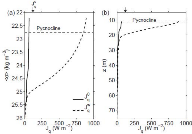
Figure 3 - (a) Average downward heat flux profiles as a function of density for background conditions (solid line) and waves (dashed line). Background conditions are based on profiles taken just prior to wave groups, and a 24 hour stationary profiling series with periods of waves removed. (b) Same as in panel (a), but plotted as a function of depth. Profiles have been filtered to include scales larger than 7 m. Arrows show the average surface heat flux.
