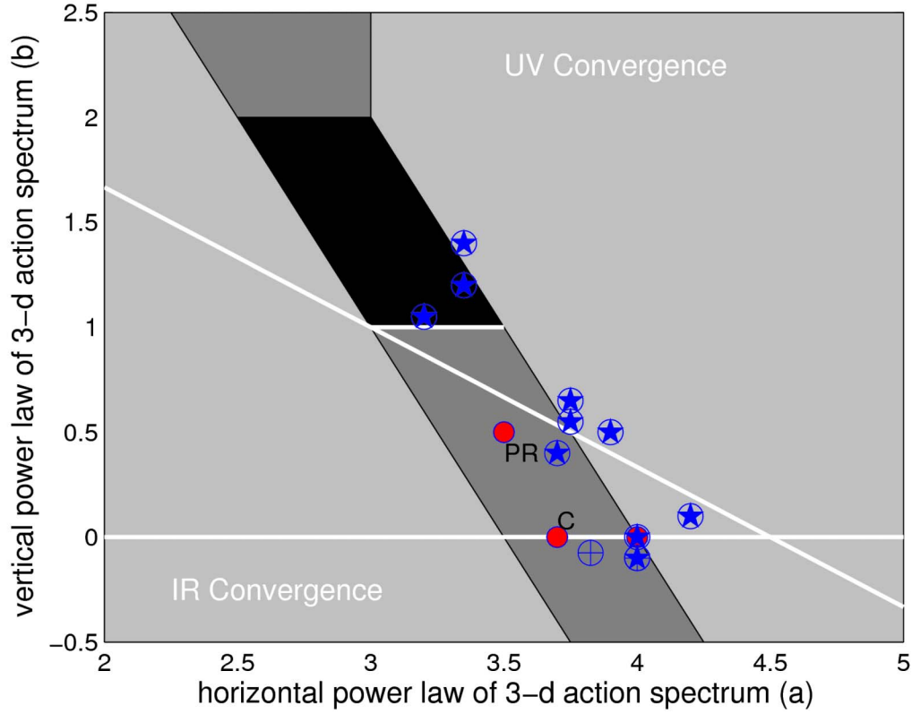
Figure Three. The observational points and the theories. The filled circles represent the Pelinovsky-Raevsky (PR) spectrum, the convergent numerical solution determined in Section 4c and the GM spectrum. Circles with stars represent power-law estimates based upon one-dimensional spectra. Circles with cross hairs represent estimates based upon two-dimensional data sets. Light grey shading represents regions of the power-law domain for which the collision integral converges in either the IR or UV limit. The dark grey shading represents the region of the power-law domain for which the IR and UV limits diverge and have opposite signs. The region of black shading represents the sub-domain for which both the IR and UV divergences have the same sign, i.e. when large contributions from interactions with very small and very large wavenumbers have the same sign. Overlain as solid white lines are the induced diffusion stationary states.
