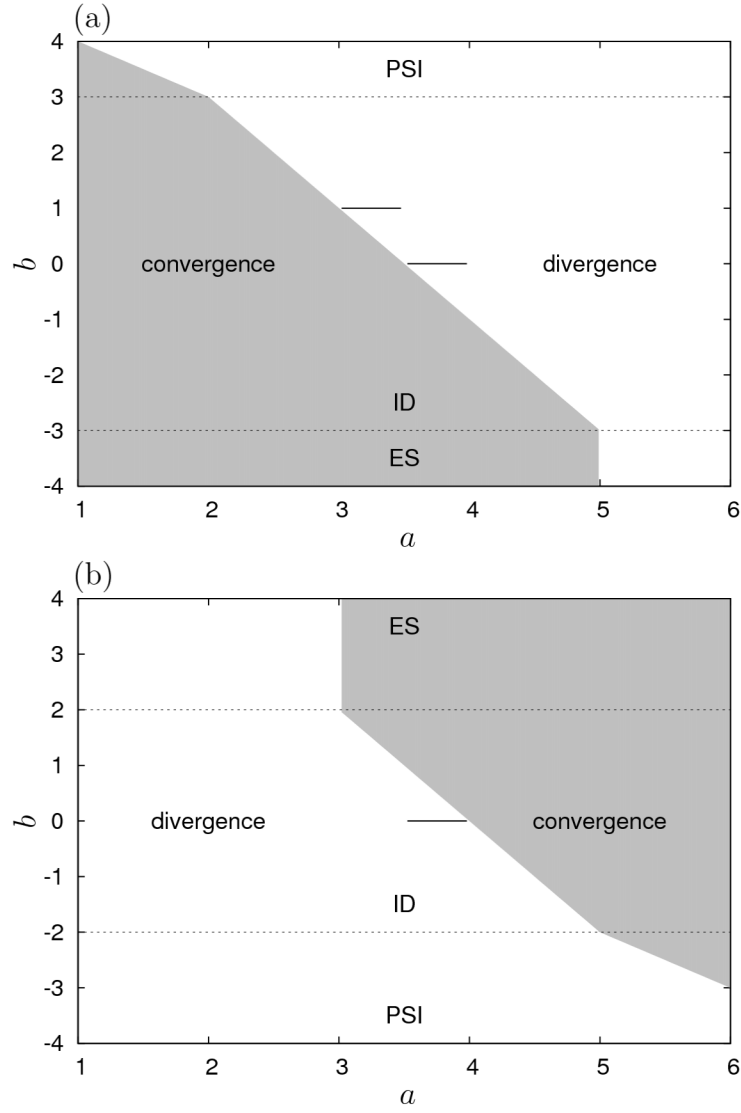
Figure One. Convergence/divergence regions of the kinetic equation. Divergence/convergence due to IR wavenumbers (a) and due to UV wavenumbers (b). The integral converge for the exponents in the shaded regions or on the segments ( b=0 , 7/2 < a < 4 ) and ( b=1 , 3 < a < 7/2 ). Dashed lines distinguish the domains where the indicated named triads dominate the singularity.
