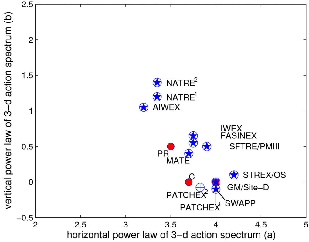
Figure Two. Observational Programs of the last four decades. The filled circles represent the Pelinovsky--Raevsky (PR) spectrum (a,b) = (3.5,0.5) , the convergent numerical solution (a,b) = (3.7,0.0) and the GM spectrum (a,b) = (4.0,0.0) . Circles with stars represent estimates based upon one-dimensional spectra. There are two estimates obtained from two-dimensional data sets represented as circles with cross hairs. The figure contains 12 observational points from 10 observational programs. Note that PATCHEX1 is indistinguishable from SWAPP. Also note that one of the three filled circles (GM) coincides with the experimental point from Site-D.
